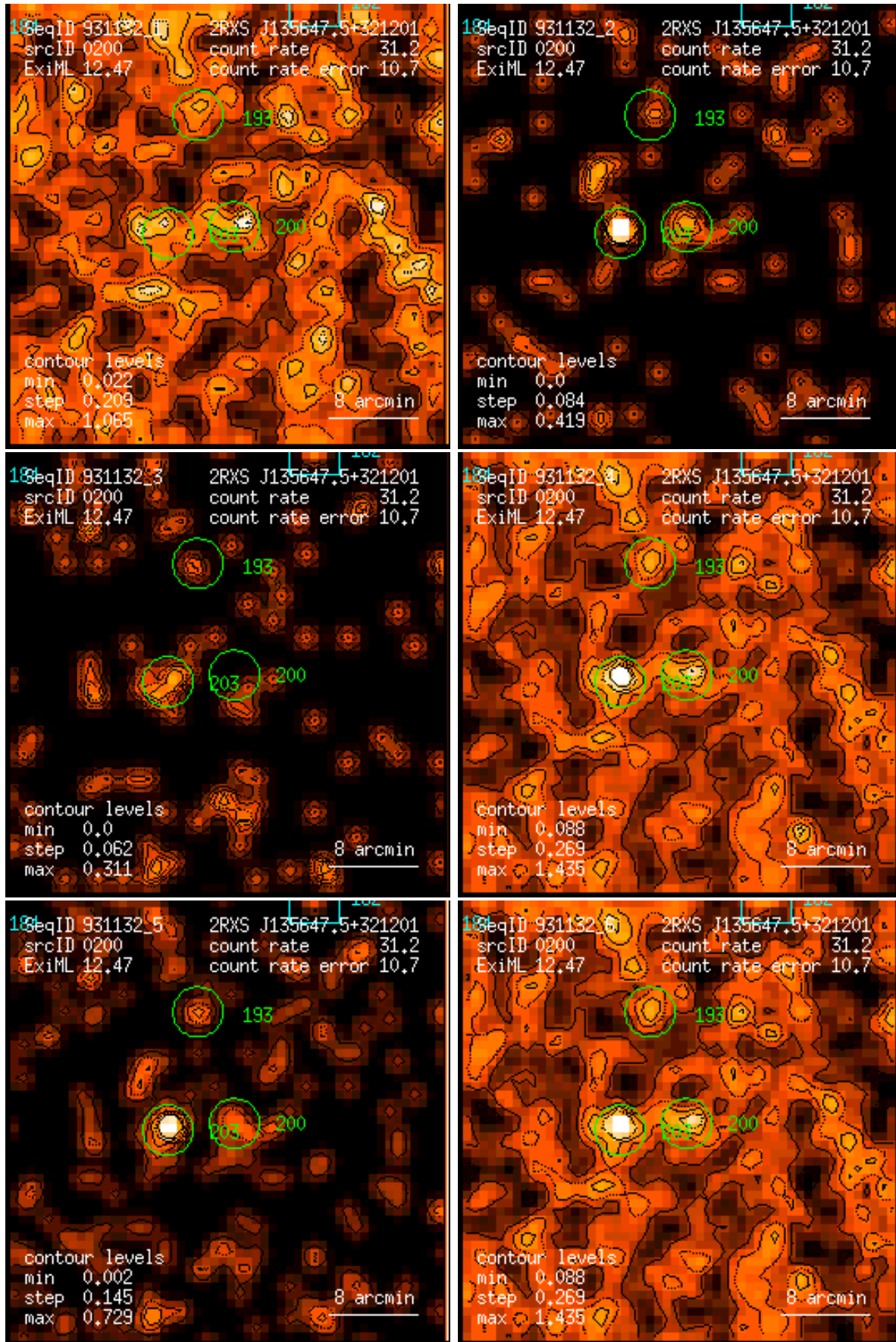
Figure 200: RASS 931132: detection 0200: band rate images, Gaussian filter: (1) PSPC channels 11 – 41, (2) 52 – 90, (3) 91 – 201, (4) 11 – 235, (5) 52 – 201, (6) 11 – 201. Broad band rates in counts/ks. Band rate contour levels in counts/ks/arcmin 2 .
