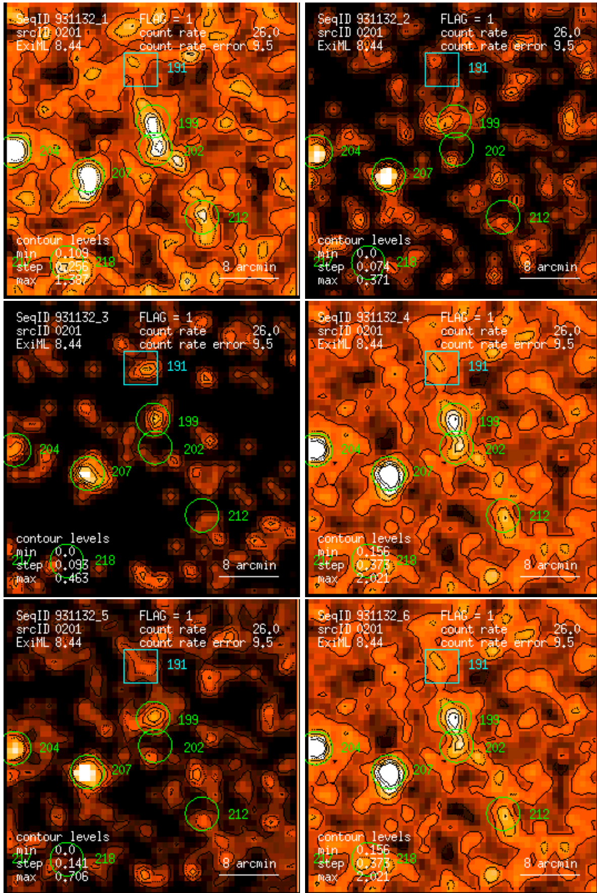
Figure 201: RASS 931132: detection 0201: band rate images, Gaussian filter: (1) PSPC channels 11 – 41, (2) 52 – 90, (3) 91 – 201, (4) 11 – 235, (5) 52 – 201, (6) 11 – 201. Broad band rates in counts/ks. Band rate contour levels in counts/ks/arcmin 2 .
