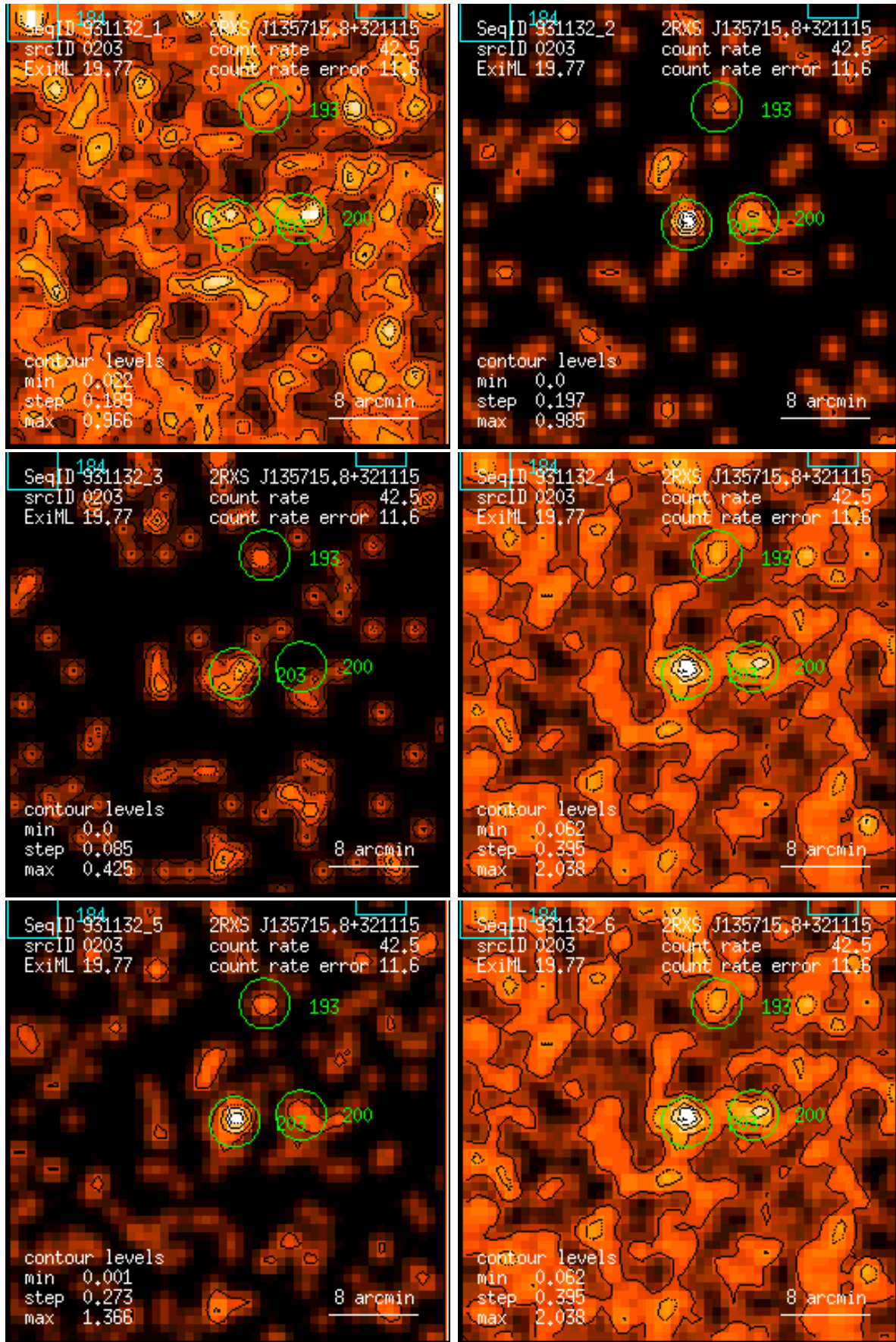
Figure 203: RASS 931132: detection 0203: band rate images, Gaussian filter: (1) PSPC channels 11 – 41, (2) 52 – 90, (3) 91 – 201, (4) 11 – 235, (5) 52 – 201, (6) 11 – 201. Broad band rates in counts/ks. Band rate contour levels in counts/ks/arcmin 2 .
