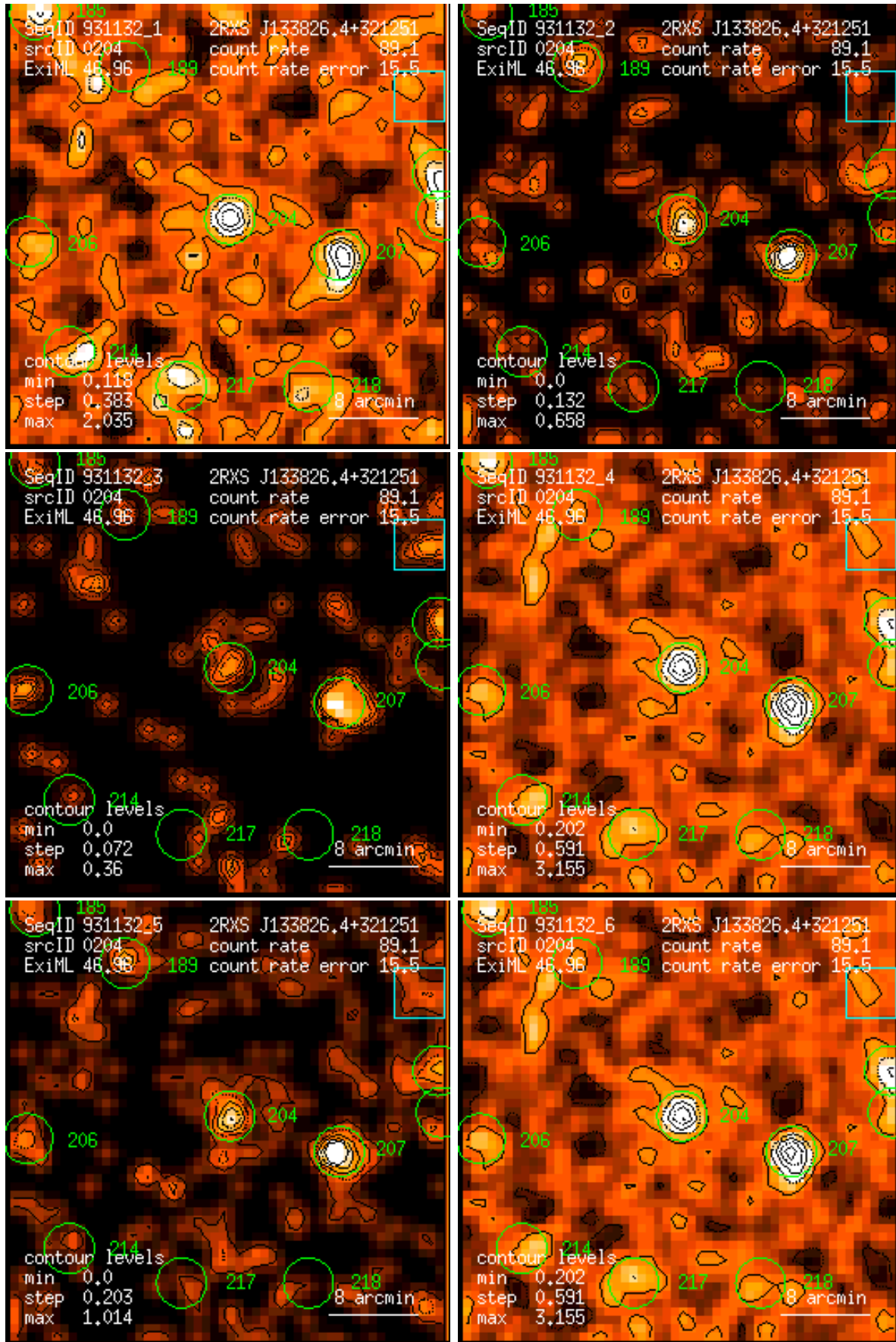
Figure 204: RASS 931132: detection 0204: band rate images, Gaussian filter: (1) PSPC channels 11 – 41, (2) 52 – 90, (3) 91 – 201, (4) 11 – 235, (5) 52 – 201, (6) 11 – 201. Broad band rates in counts/ks. Band rate contour levels in counts/ks/arcmin 2 .
