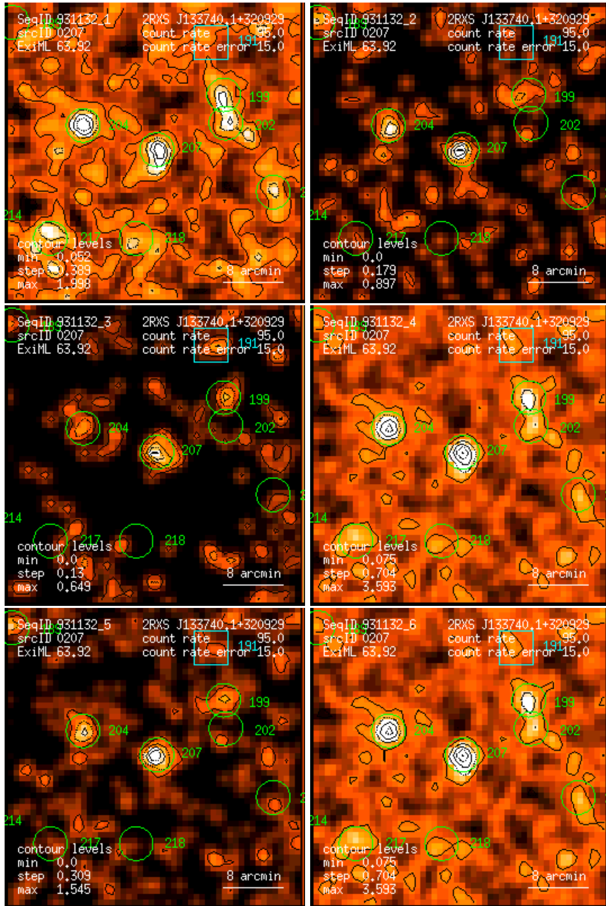
Figure 207: RASS 931132: detection 0207: band rate images, Gaussian filter: (1) PSPC channels 11 – 41, (2) 52 – 90, (3) 91 – 201, (4) 11 – 235, (5) 52 – 201, (6) 11 – 201. Broad band rates in counts/ks. Band rate contour levels in counts/ks/arcmin 2 .
