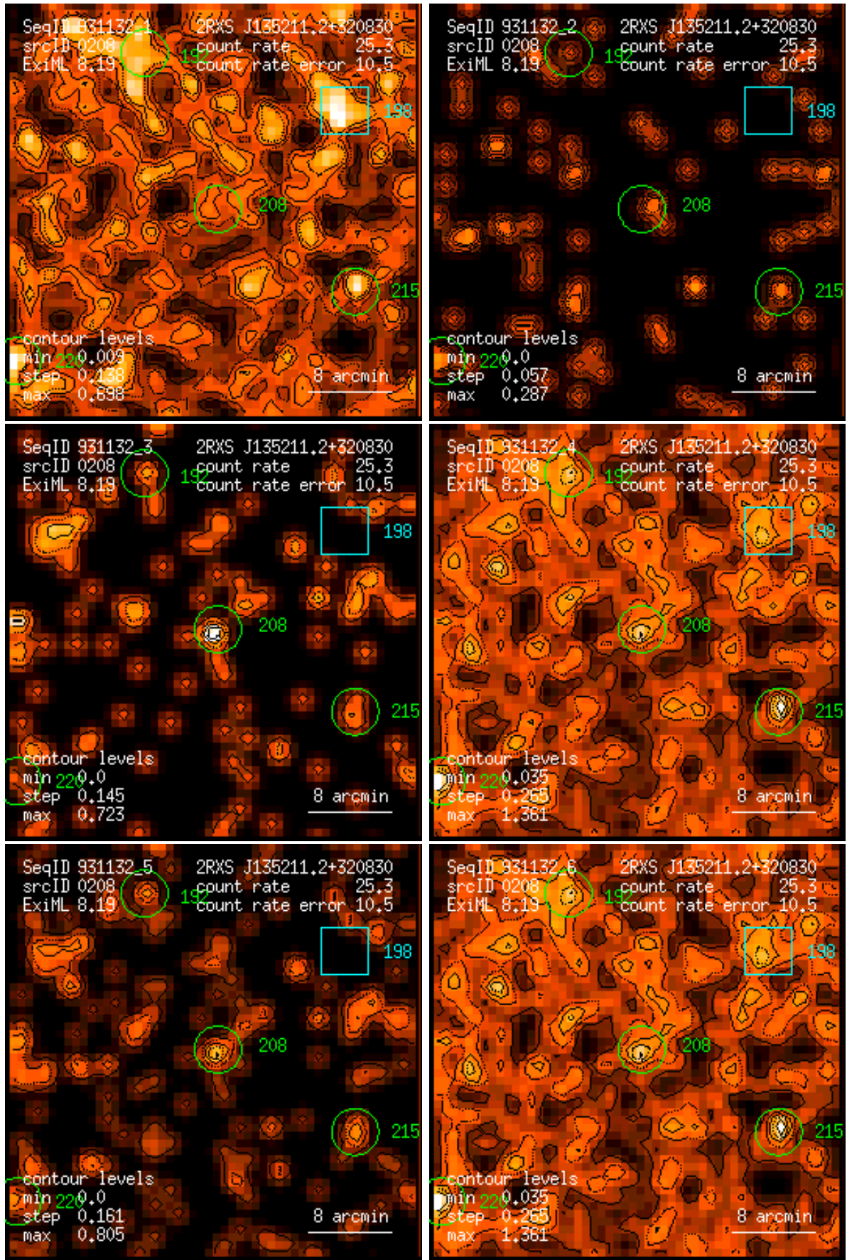
Figure 208: RASS 931132: detection 0208: band rate images, Gaussian filter: (1) PSPC channels 11 – 41, (2) 52 – 90, (3) 91 – 201, (4) 11 – 235, (5) 52 – 201, (6) 11 – 201. Broad band rates in counts/ks. Band rate contour levels in counts/ks/arcmin 2 .
