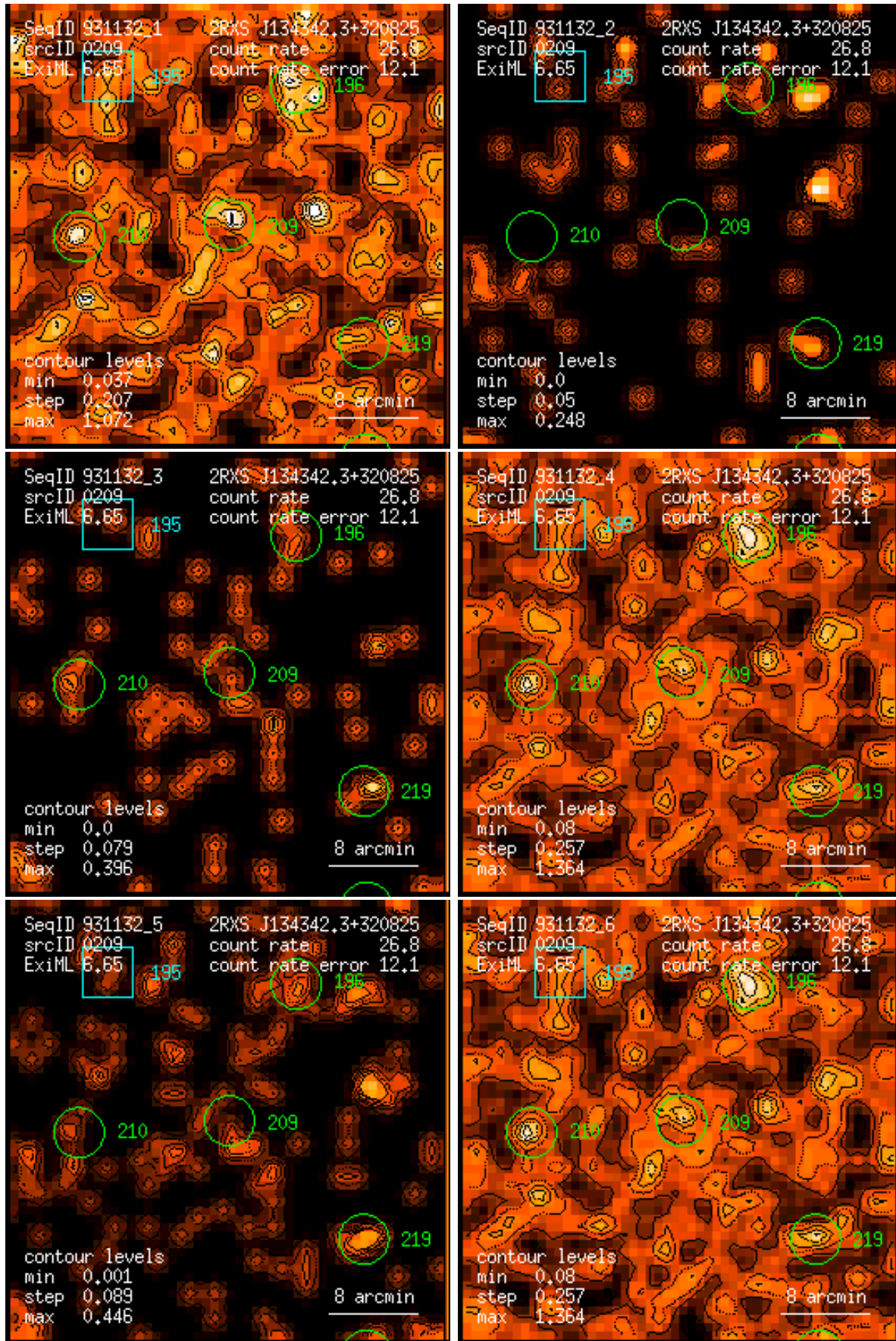
Figure 209: RASS 931132: detection 0209: band rate images, Gaussian filter: (1) PSPC channels 11 – 41, (2) 52 – 90, (3) 91 – 201, (4) 11 – 235, (5) 52 – 201, (6) 11 – 201. Broad band rates in counts/ks. Band rate contour levels in counts/ks/arcmin 2 .
