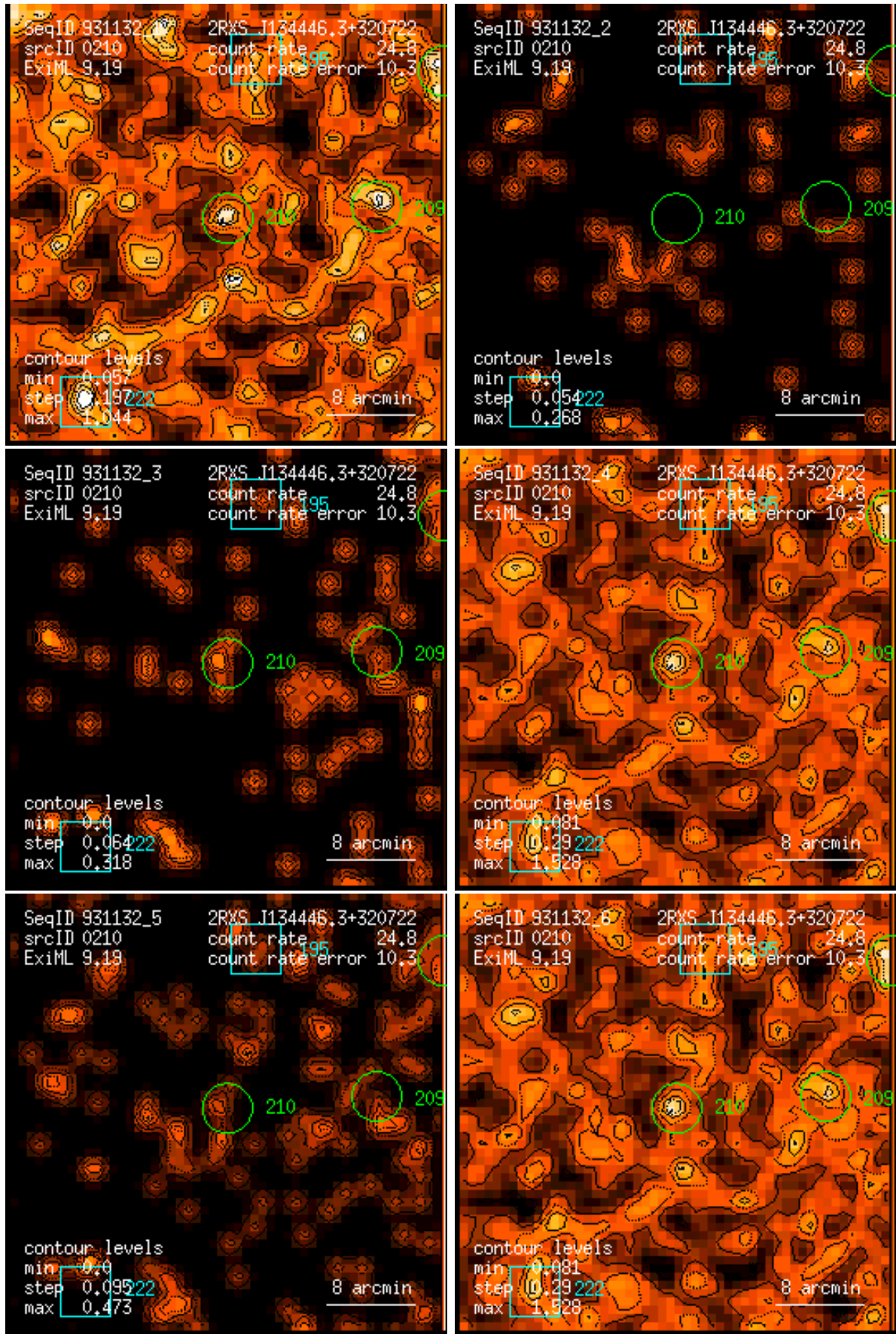
Figure 210: RASS 931132: detection 0210: band rate images, Gaussian filter: (1) PSPC channels 11 – 41, (2) 52 – 90, (3) 91 – 201, (4) 11 – 235, (5) 52 – 201, (6) 11 – 201. Broad band rates in counts/ks. Band rate contour levels in counts/ks/arcmin 2 .
