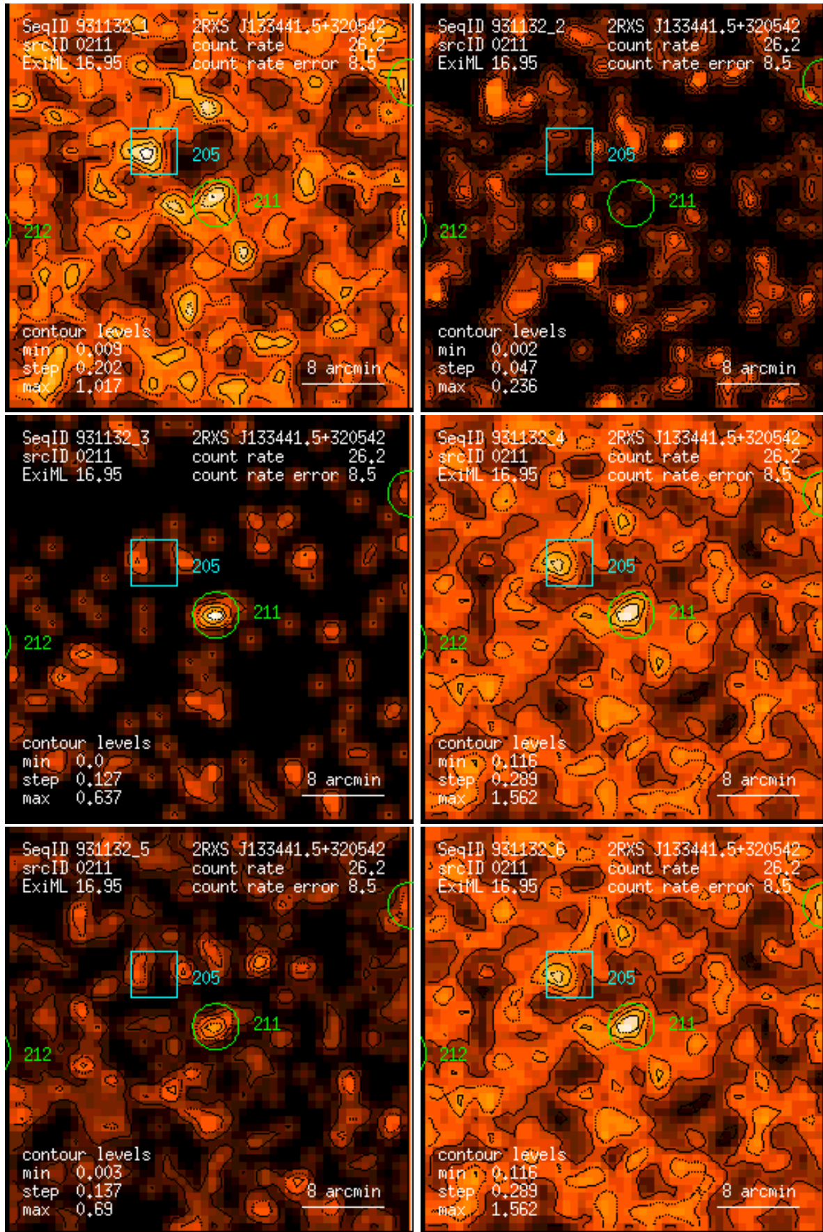
Figure 211: RASS 931132: detection 0211: band rate images, Gaussian filter: (1) PSPC channels 11 – 41, (2) 52 – 90, (3) 91 – 201, (4) 11 – 235, (5) 52 – 201, (6) 11 – 201. Broad band rates in counts/ks. Band rate contour levels in counts/ks/arcmin 2 .
