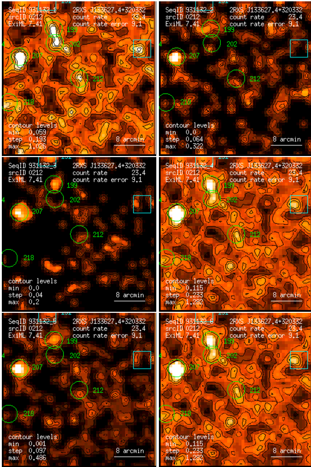
Figure 212: RASS 931132: detection 0212: band rate images, Gaussian filter: (1) PSPC channels 11 – 41, (2) 52 – 90, (3) 91 – 201, (4) 11 – 235, (5) 52 – 201, (6) 11 – 201. Broad band rates in counts/ks. Band rate contour levels in counts/ks/arcmin 2 .
