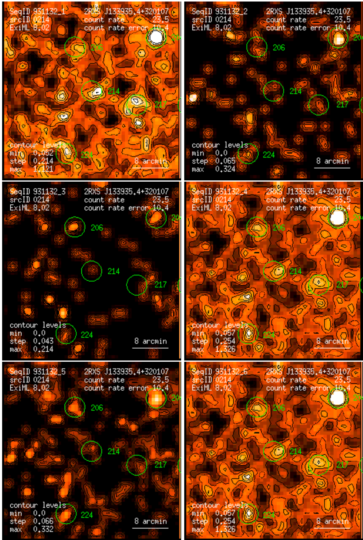
Figure 214: RASS 931132: detection 0214: band rate images, Gaussian filter: (1) PSPC channels 11 – 41, (2) 52 – 90, (3) 91 – 201, (4) 11 – 235, (5) 52 – 201, (6) 11 – 201. Broad band rates in counts/ks. Band rate contour levels in counts/ks/arcmin 2 .
