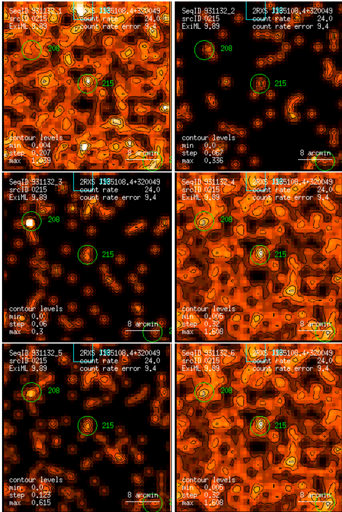
Figure 215: RASS 931132: detection 0215: band rate images, Gaussian filter: (1) PSPC channels 11 – 41, (2) 52 – 90, (3) 91 – 201, (4) 11 – 235, (5) 52 – 201, (6) 11 – 201. Broad band rates in counts/ks. Band rate contour levels in counts/ks/arcmin 2 .
