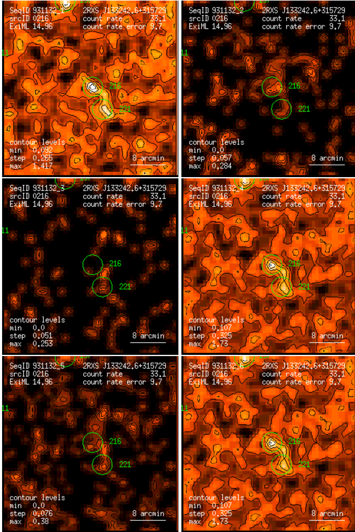
Figure 216: RASS 931132: detection 0216: band rate images, Gaussian filter: (1) PSPC channels 11 – 41, (2) 52 – 90, (3) 91 – 201, (4) 11 – 235, (5) 52 – 201, (6) 11 – 201. Broad band rates in counts/ks. Band rate contour levels in counts/ks/arcmin 2 .
