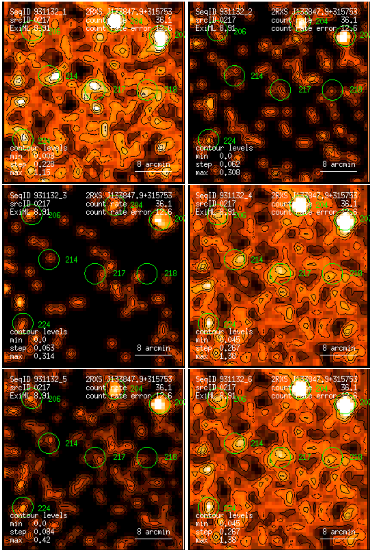
Figure 217: RASS 931132: detection 0217: band rate images, Gaussian filter: (1) PSPC channels 11 – 41, (2) 52 – 90, (3) 91 – 201, (4) 11 – 235, (5) 52 – 201, (6) 11 – 201. Broad band rates in counts/ks. Band rate contour levels in counts/ks/arcmin 2 .
