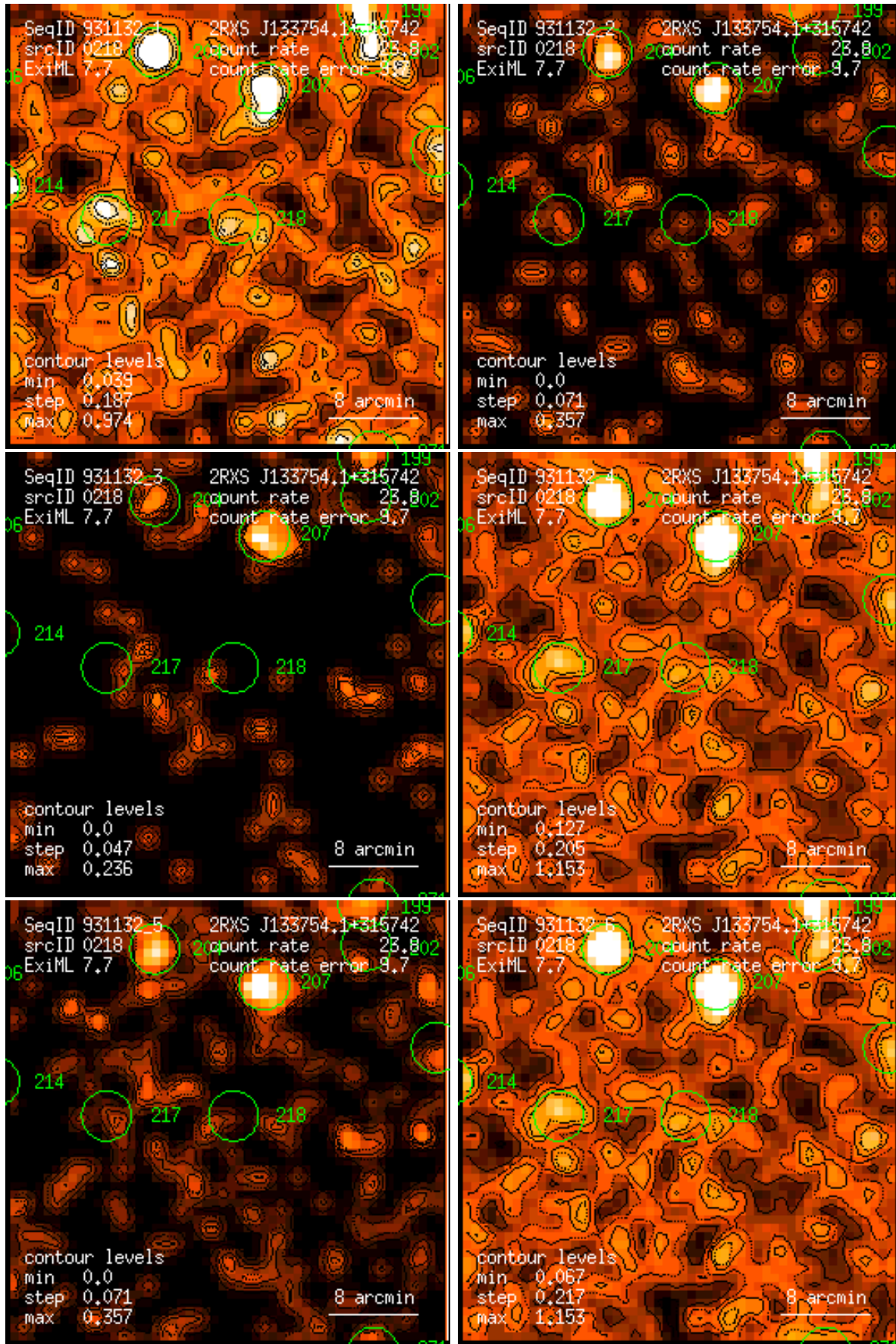
Figure 218: RASS 931132: detection 0218: band rate images, Gaussian filter: (1) PSPC channels 11 – 41, (2) 52 – 90, (3) 91 – 201, (4) 11 – 235, (5) 52 – 201, (6) 11 – 201. Broad band rates in counts/ks. Band rate contour levels in counts/ks/arcmin 2 .
