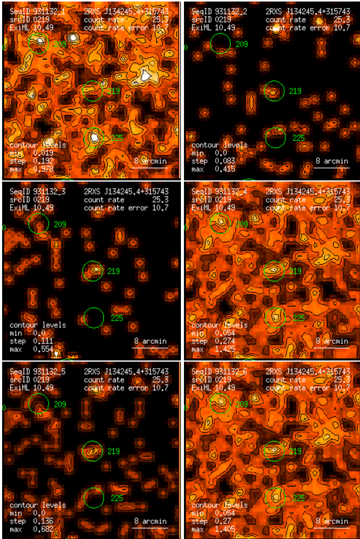
Figure 219: RASS 931132: detection 0219: band rate images, Gaussian filter: (1) PSPC channels 11 – 41, (2) 52 – 90, (3) 91 – 201, (4) 11 – 235, (5) 52 – 201, (6) 11 – 201. Broad band rates in counts/ks. Band rate contour levels in counts/ks/arcmin 2 .
