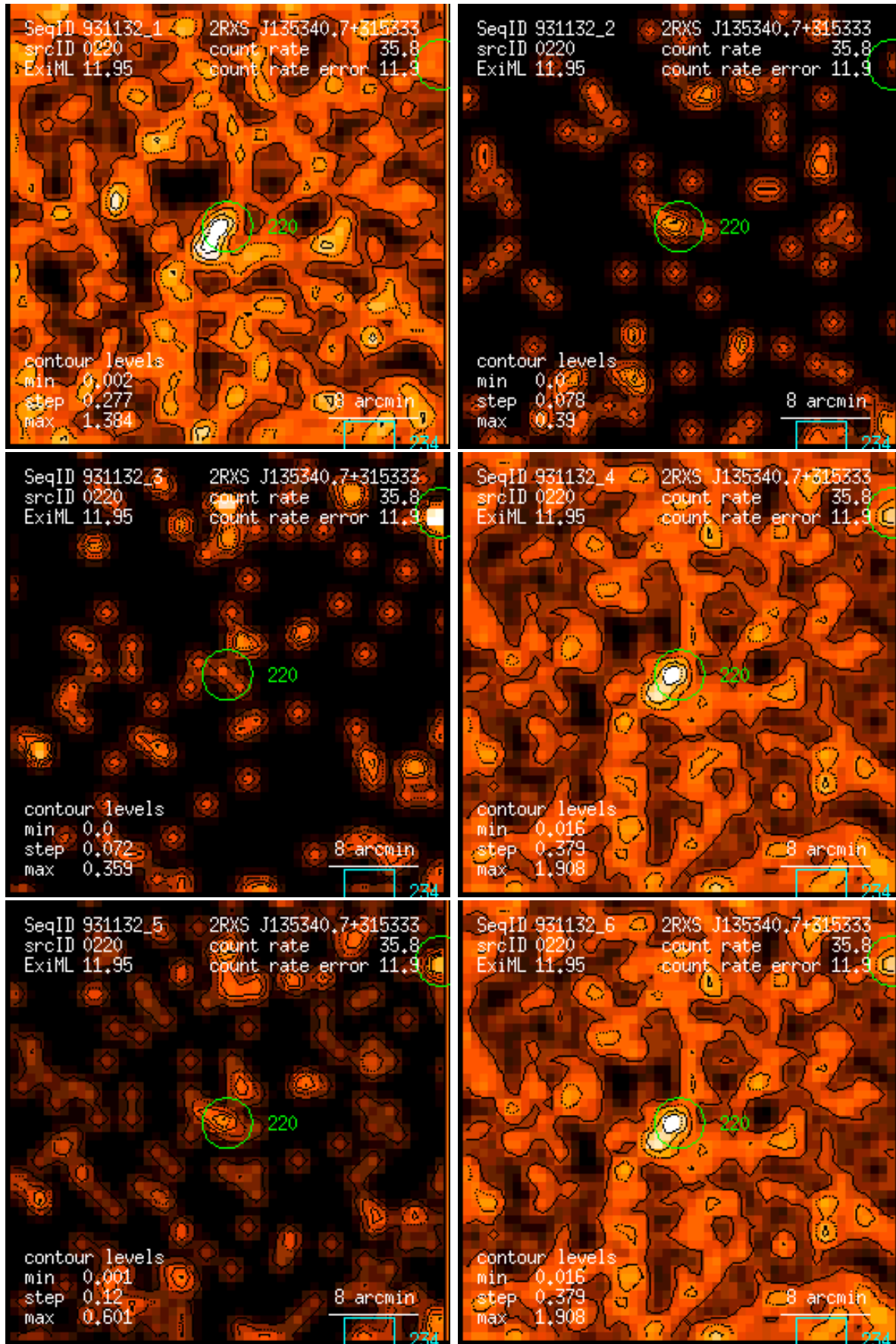
Figure 220: RASS 931132: detection 0220: band rate images, Gaussian filter: (1) PSPC channels 11 – 41, (2) 52 – 90, (3) 91 – 201, (4) 11 – 235, (5) 52 – 201, (6) 11 – 201. Broad band rates in counts/ks. Band rate contour levels in counts/ks/arcmin 2 .
