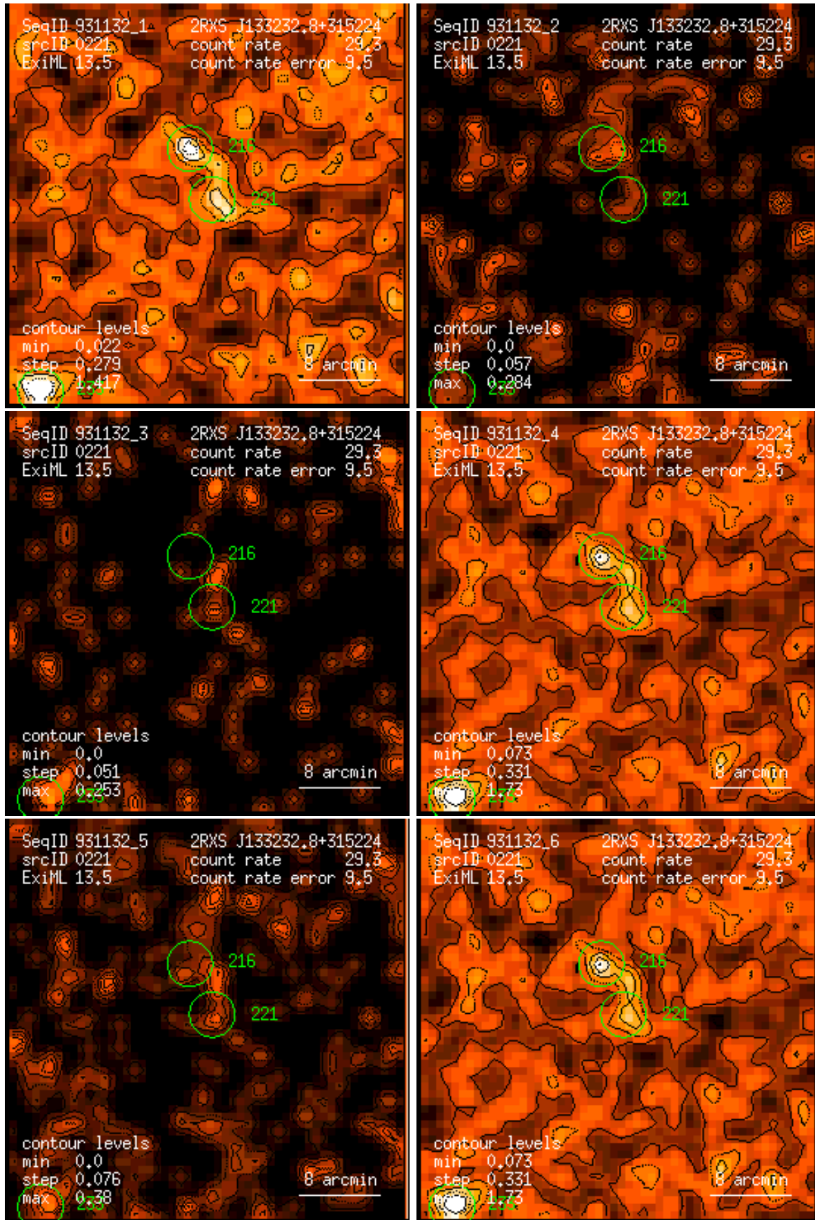
Figure 221: RASS 931132: detection 0221: band rate images, Gaussian filter: (1) PSPC channels 11 – 41, (2) 52 – 90, (3) 91 – 201, (4) 11 – 235, (5) 52 – 201, (6) 11 – 201. Broad band rates in counts/ks. Band rate contour levels in counts/ks/arcmin 2 .
