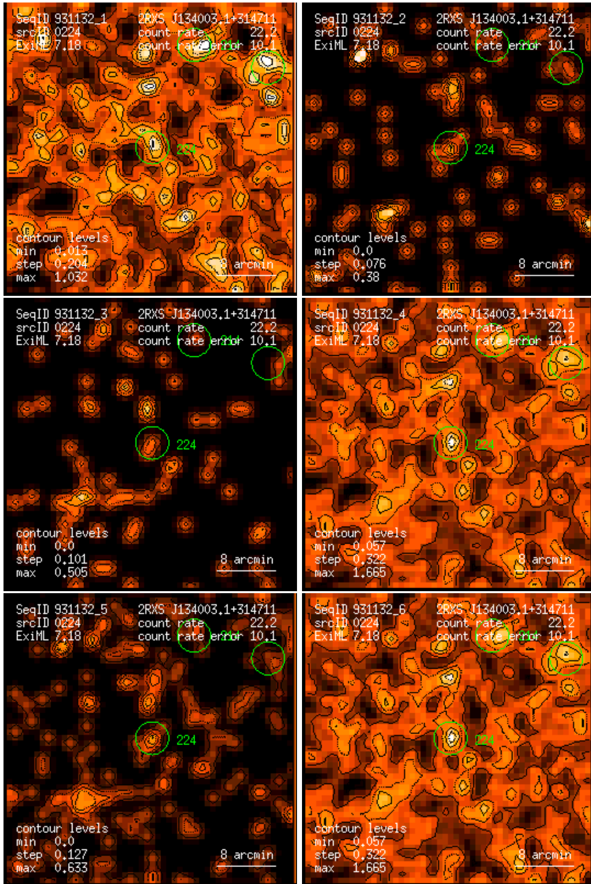
Figure 224: RASS 931132: detection 0224: band rate images, Gaussian filter: (1) PSPC channels 11 – 41, (2) 52 – 90, (3) 91 – 201, (4) 11 – 235, (5) 52 – 201, (6) 11 – 201. Broad band rates in counts/ks. Band rate contour levels in counts/ks/arcmin 2 .
