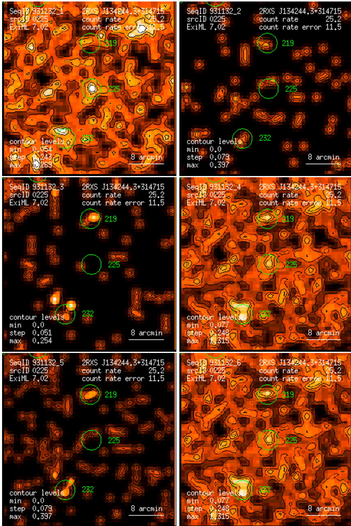
Figure 225: RASS 931132: detection 0225: band rate images, Gaussian filter: (1) PSPC channels 11 – 41, (2) 52 – 90, (3) 91 – 201, (4) 11 – 235, (5) 52 – 201, (6) 11 – 201. Broad band rates in counts/ks. Band rate contour levels in counts/ks/arcmin 2 .
