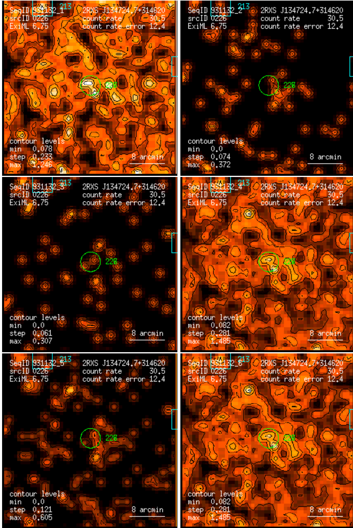
Figure 226: RASS 931132: detection 0226: band rate images, Gaussian filter: (1) PSPC channels 11 – 41, (2) 52 – 90, (3) 91 – 201, (4) 11 – 235, (5) 52 – 201, (6) 11 – 201. Broad band rates in counts/ks. Band rate contour levels in counts/ks/arcmin 2 .
