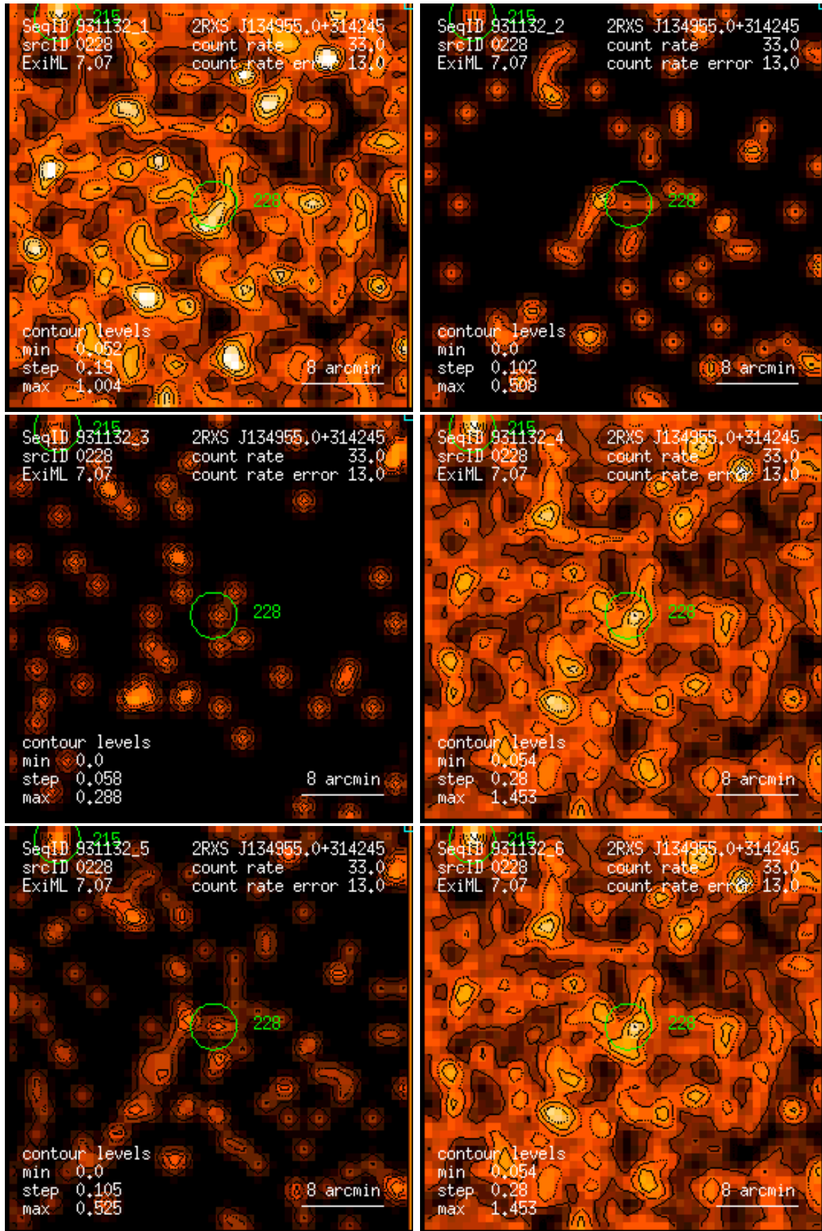
Figure 228: RASS 931132: detection 0228: band rate images, Gaussian filter: (1) PSPC channels 11 – 41, (2) 52 – 90, (3) 91 – 201, (4) 11 – 235, (5) 52 – 201, (6) 11 – 201. Broad band rates in counts/ks. Band rate contour levels in counts/ks/arcmin 2 .
