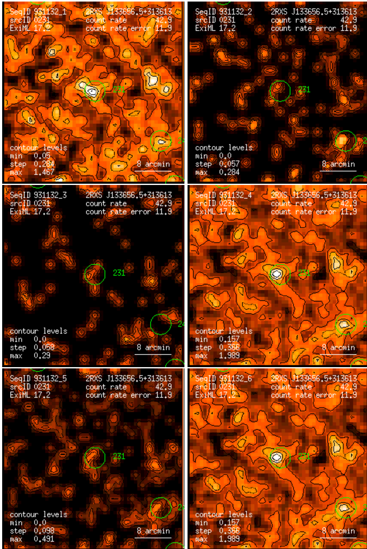
Figure 231: RASS 931132: detection 0231: band rate images, Gaussian filter: (1) PSPC channels 11 – 41, (2) 52 – 90, (3) 91 – 201, (4) 11 – 235, (5) 52 – 201, (6) 11 – 201. Broad band rates in counts/ks. Band rate contour levels in counts/ks/arcmin 2 .
