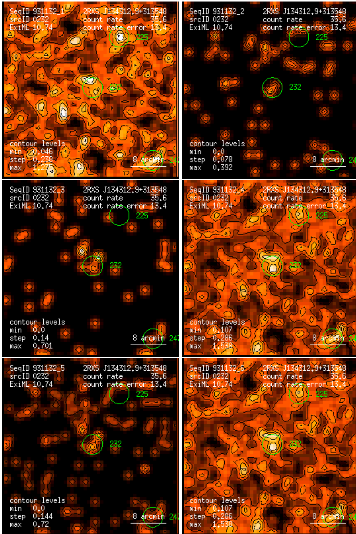
Figure 232: RASS 931132: detection 0232: band rate images, Gaussian filter: (1) PSPC channels 11 – 41, (2) 52 – 90, (3) 91 – 201, (4) 11 – 235, (5) 52 – 201, (6) 11 – 201. Broad band rates in counts/ks. Band rate contour levels in counts/ks/arcmin 2 .
