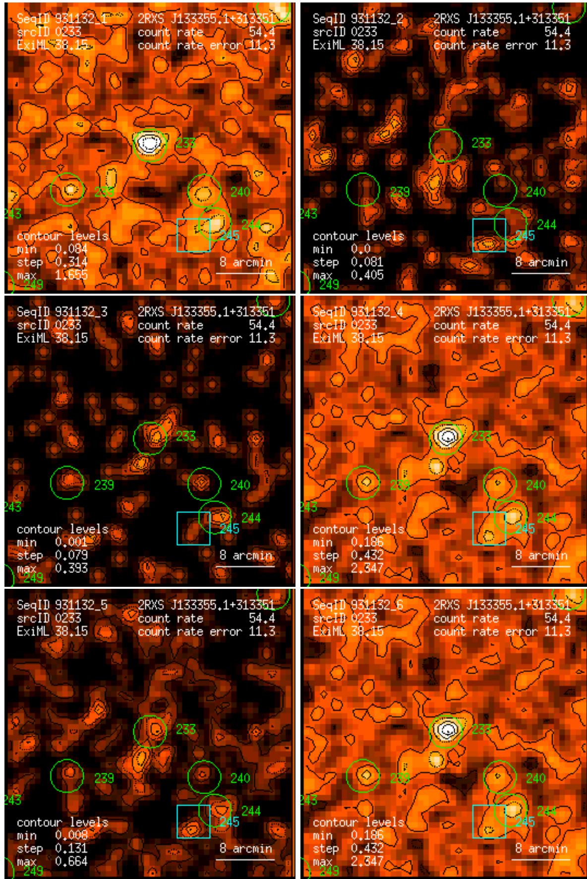
Figure 233: RASS 931132: detection 0233: band rate images, Gaussian filter: (1) PSPC channels 11 – 41, (2) 52 – 90, (3) 91 – 201, (4) 11 – 235, (5) 52 – 201, (6) 11 – 201. Broad band rates in counts/ks. Band rate contour levels in counts/ks/arcmin 2 .
