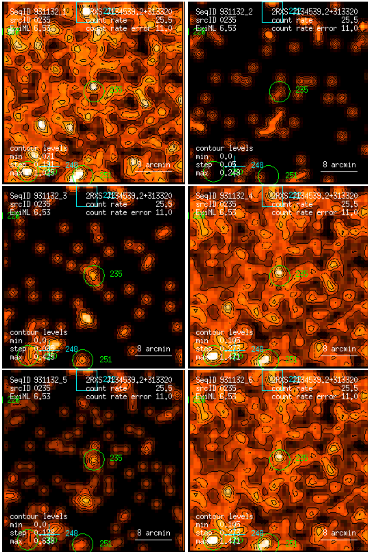
Figure 235: RASS 931132: detection 0235: band rate images, Gaussian filter: (1) PSPC channels 11 – 41, (2) 52 – 90, (3) 91 – 201, (4) 11 – 235, (5) 52 – 201, (6) 11 – 201. Broad band rates in counts/ks. Band rate contour levels in counts/ks/arcmin 2 .
