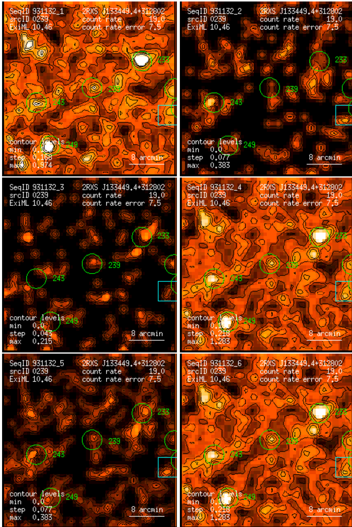
Figure 239: RASS 931132: detection 0239: band rate images, Gaussian filter: (1) PSPC channels 11 – 41, (2) 52 – 90, (3) 91 – 201, (4) 11 – 235, (5) 52 – 201, (6) 11 – 201. Broad band rates in counts/ks. Band rate contour levels in counts/ks/arcmin 2 .
