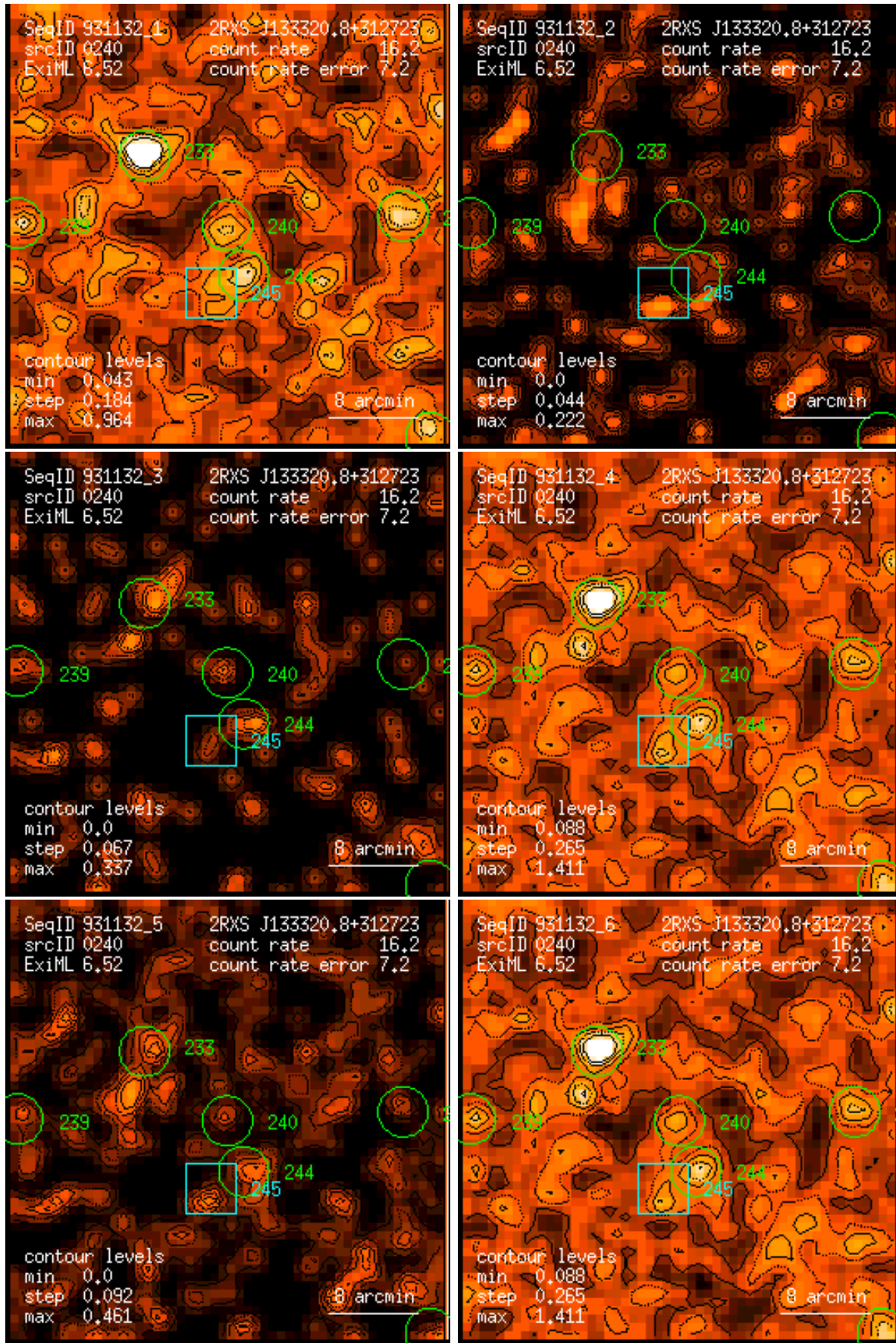
Figure 240: RASS 931132: detection 0240: band rate images, Gaussian filter: (1) PSPC channels 11 – 41, (2) 52 – 90, (3) 91 – 201, (4) 11 – 235, (5) 52 – 201, (6) 11 – 201. Broad band rates in counts/ks. Band rate contour levels in counts/ks/arcmin 2 .
