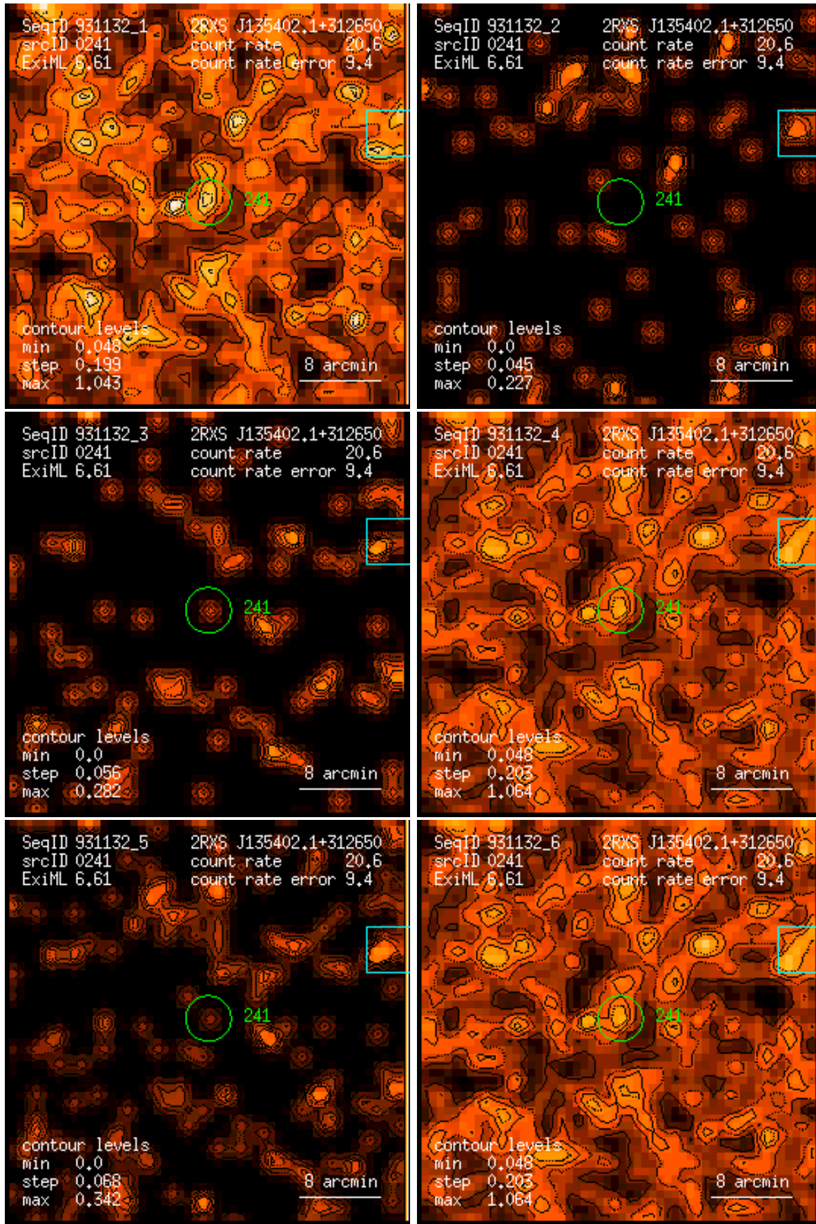
Figure 241: RASS 931132: detection 0241: band rate images, Gaussian filter: (1) PSPC channels 11 – 41, (2) 52 – 90, (3) 91 – 201, (4) 11 – 235, (5) 52 – 201, (6) 11 – 201. Broad band rates in counts/ks. Band rate contour levels in counts/ks/arcmin 2 .
