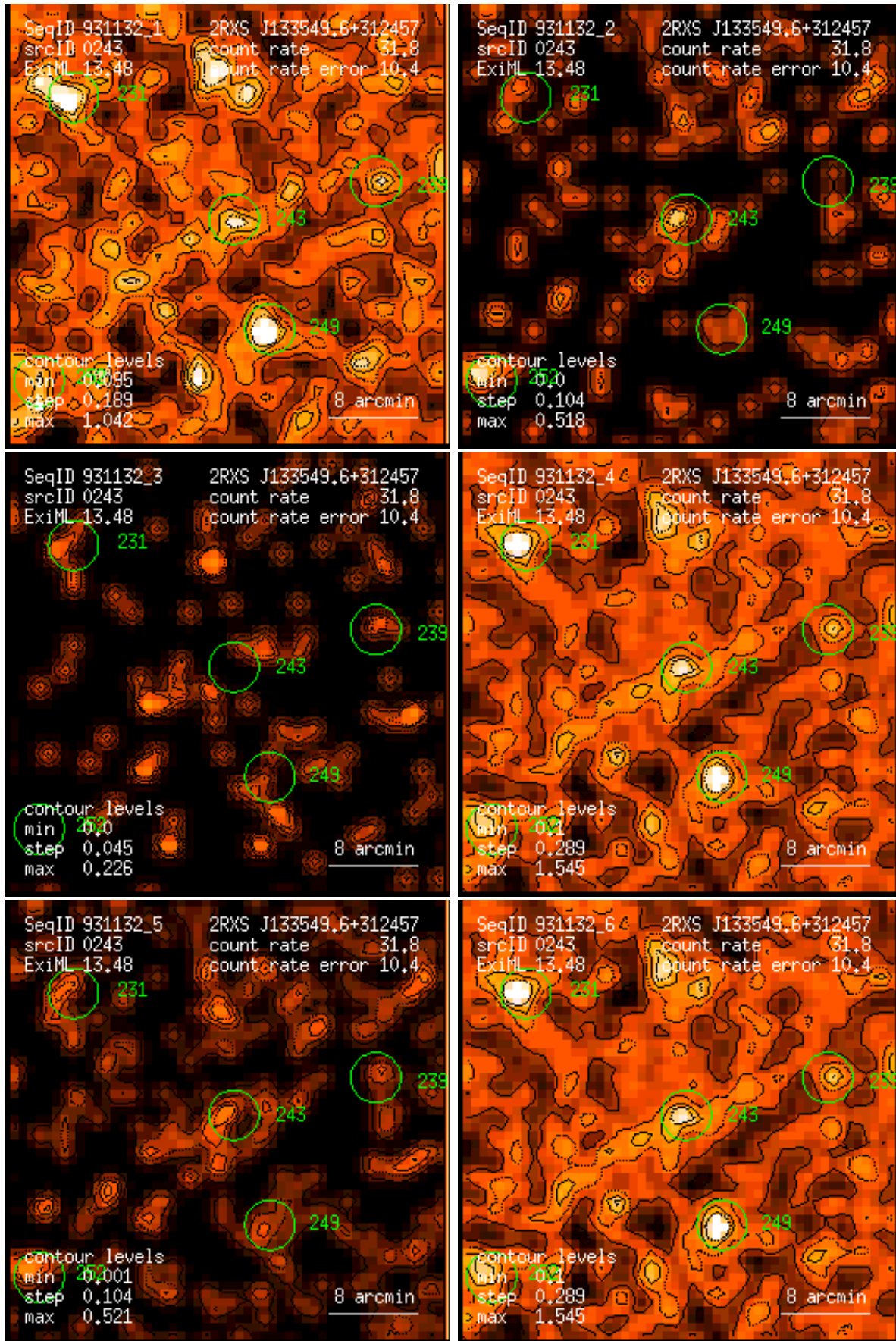
Figure 243: RASS 931132: detection 0243: band rate images, Gaussian filter: (1) PSPC channels 11 – 41, (2) 52 – 90, (3) 91 – 201, (4) 11 – 235, (5) 52 – 201, (6) 11 – 201. Broad band rates in counts/ks. Band rate contour levels in counts/ks/arcmin 2 .
