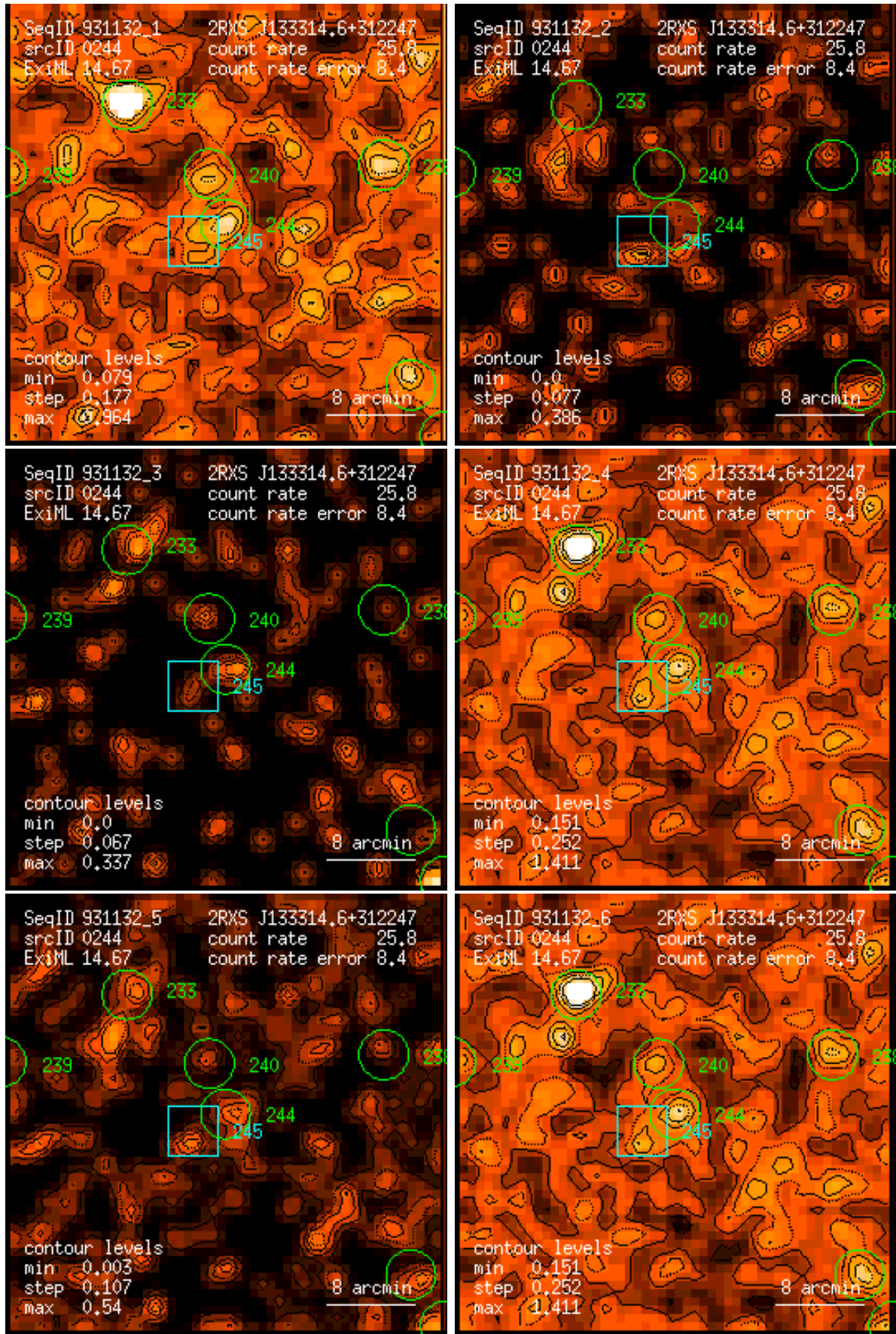
Figure 244: RASS 931132: detection 0244: band rate images, Gaussian filter: (1) PSPC channels 11 – 41, (2) 52 – 90, (3) 91 – 201, (4) 11 – 235, (5) 52 – 201, (6) 11 – 201. Broad band rates in counts/ks. Band rate contour levels in counts/ks/arcmin 2 .
