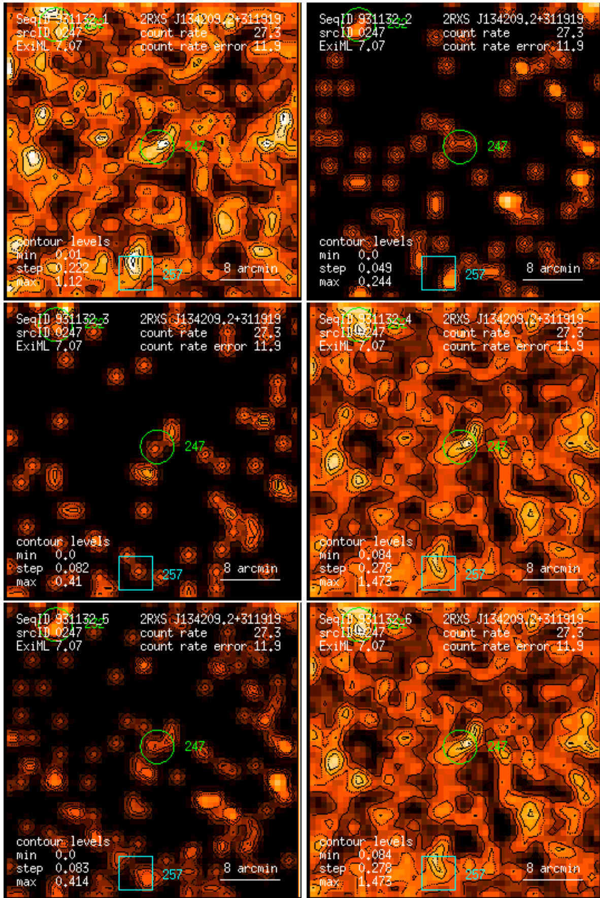
Figure 247: RASS 931132: detection 0247: band rate images, Gaussian filter: (1) PSPC channels 11 – 41, (2) 52 – 90, (3) 91 – 201, (4) 11 – 235, (5) 52 – 201, (6) 11 – 201. Broad band rates in counts/ks. Band rate contour levels in counts/ks/arcmin 2 .
