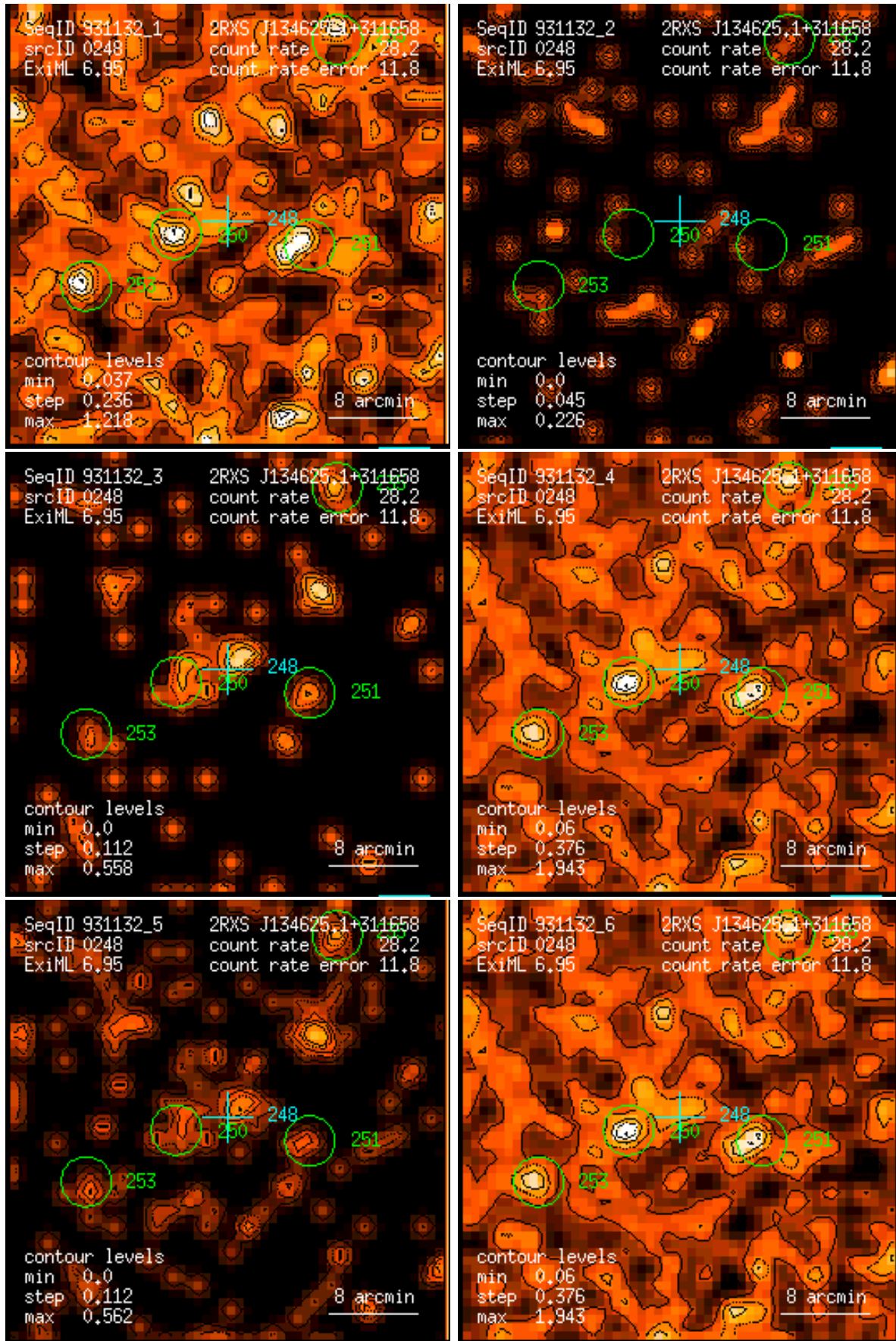
Figure 248: RASS 931132: detection 0248: band rate images, Gaussian filter: (1) PSPC channels 11 – 41, (2) 52 – 90, (3) 91 – 201, (4) 11 – 235, (5) 52 – 201, (6) 11 – 201. Broad band rates in counts/ks. Band rate contour levels in counts/ks/arcmin 2 .
