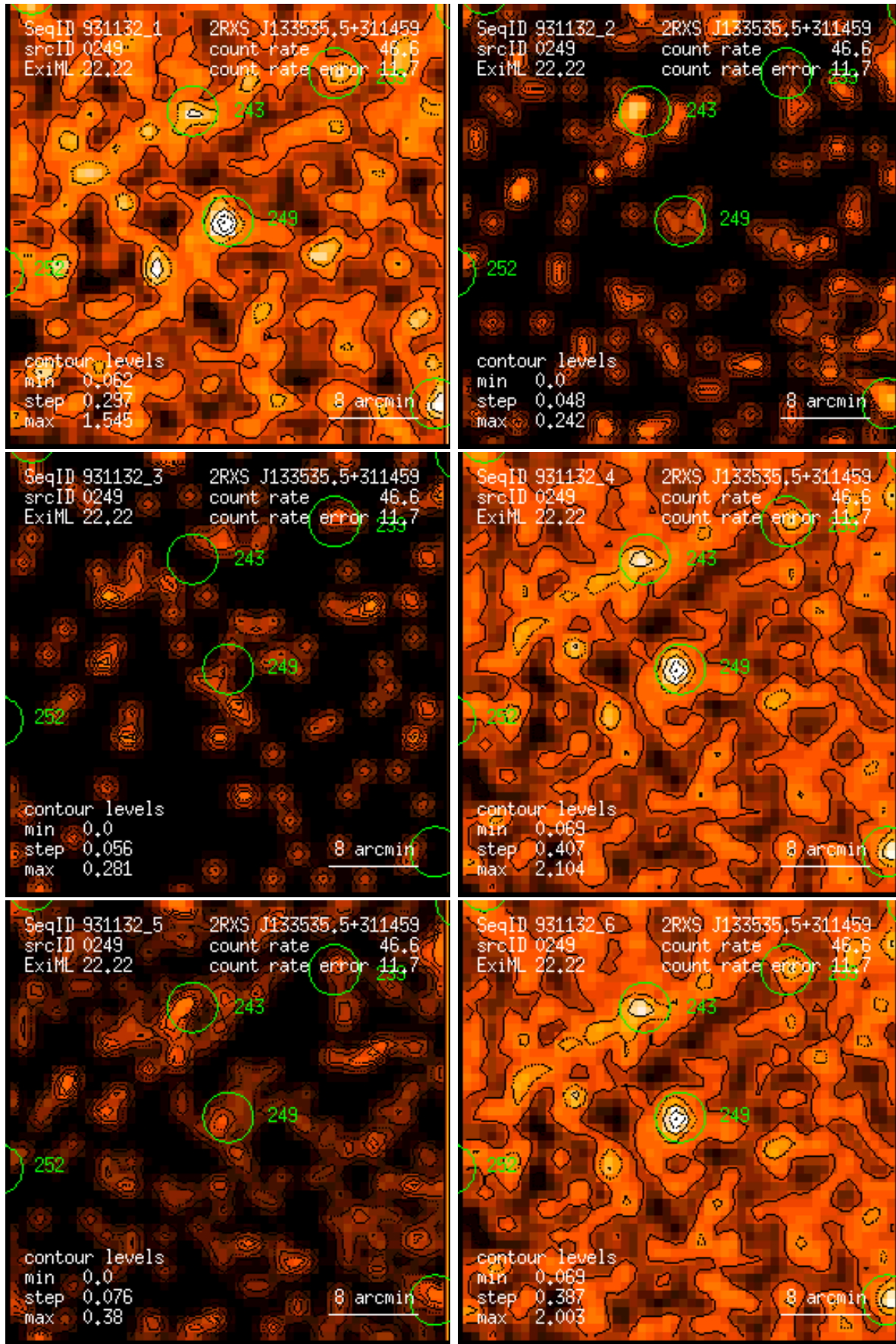
Figure 249: RASS 931132: detection 0249: band rate images, Gaussian filter: (1) PSPC channels 11 – 41, (2) 52 – 90, (3) 91 – 201, (4) 11 – 235, (5) 52 – 201, (6) 11 – 201. Broad band rates in counts/ks. Band rate contour levels in counts/ks/arcmin 2 .
