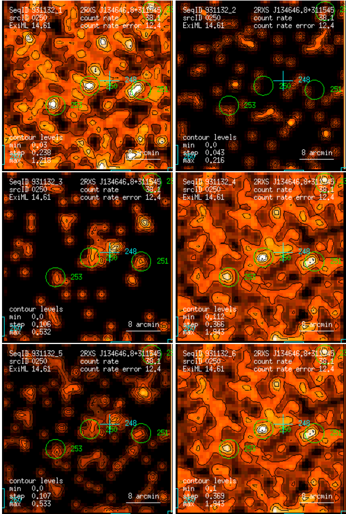
Figure 250: RASS 931132: detection 0250: band rate images, Gaussian filter: (1) PSPC channels 11 – 41, (2) 52 – 90, (3) 91 – 201, (4) 11 – 235, (5) 52 – 201, (6) 11 – 201. Broad band rates in counts/ks. Band rate contour levels in counts/ks/arcmin 2 .
