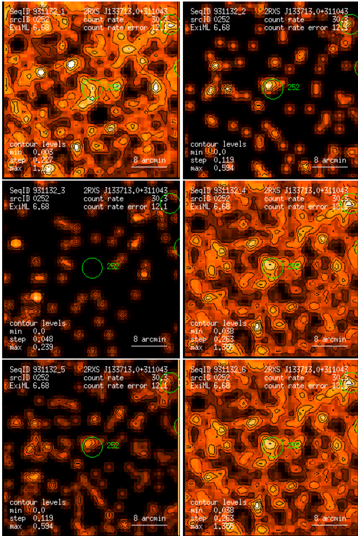
Figure 252: RASS 931132: detection 0252: band rate images, Gaussian filter: (1) PSPC channels 11 – 41, (2) 52 – 90, (3) 91 – 201, (4) 11 – 235, (5) 52 – 201, (6) 11 – 201. Broad band rates in counts/ks. Band rate contour levels in counts/ks/arcmin 2 .
