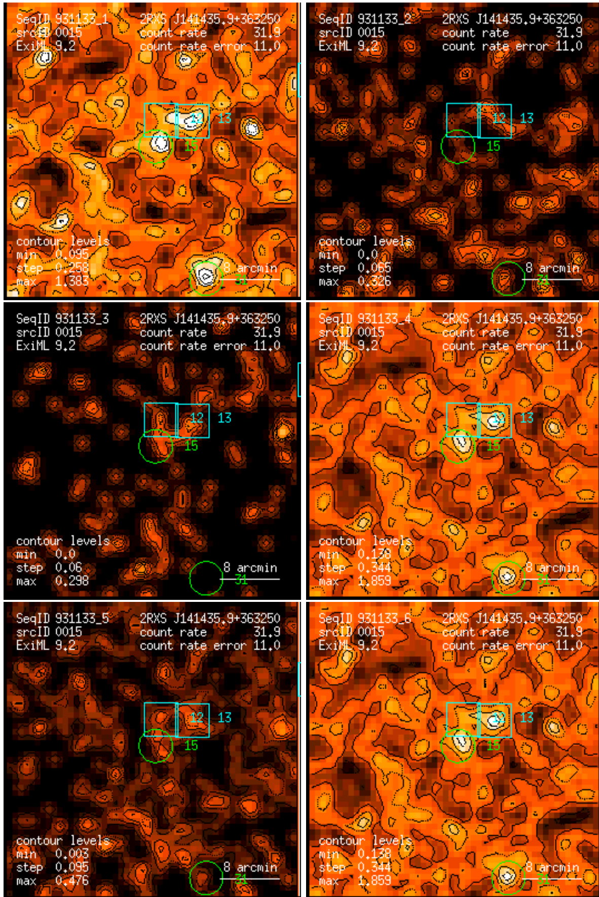
Figure 15: RASS 931133: detection 0015: band rate images, Gaussian filter: (1) PSPC channels 11 – 41, (2) 52 – 90, (3) 91 – 201, (4) 11 – 235, (5) 52 – 201, (6) 11 – 201. Broad band rates in counts/ks. Band rate contour levels in counts/ks/arcmin 2 .
