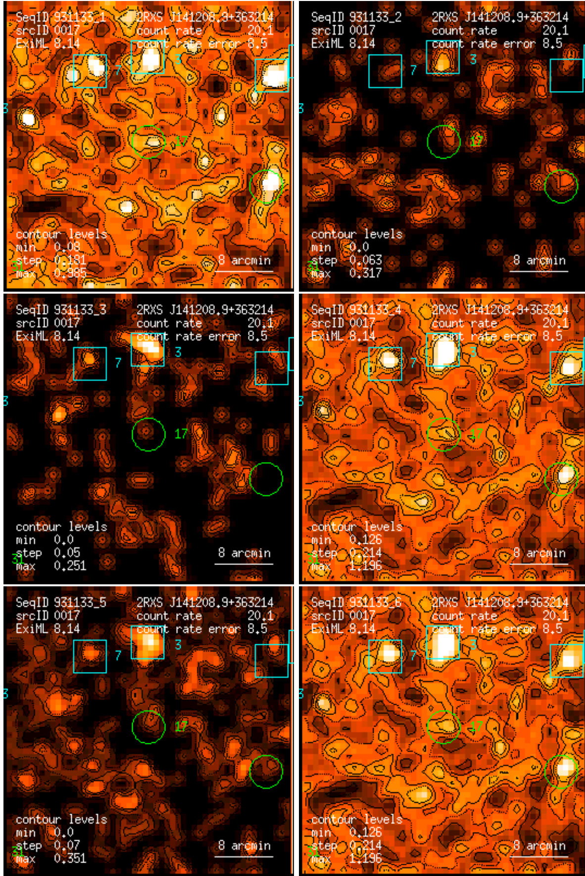
Figure 17: RASS 931133: detection 0017: band rate images, Gaussian filter: (1) PSPC channels 11 – 41, (2) 52 – 90, (3) 91 – 201, (4) 11 – 235, (5) 52 – 201, (6) 11 – 201. Broad band rates in counts/ks. Band rate contour levels in counts/ks/arcmin 2 .
