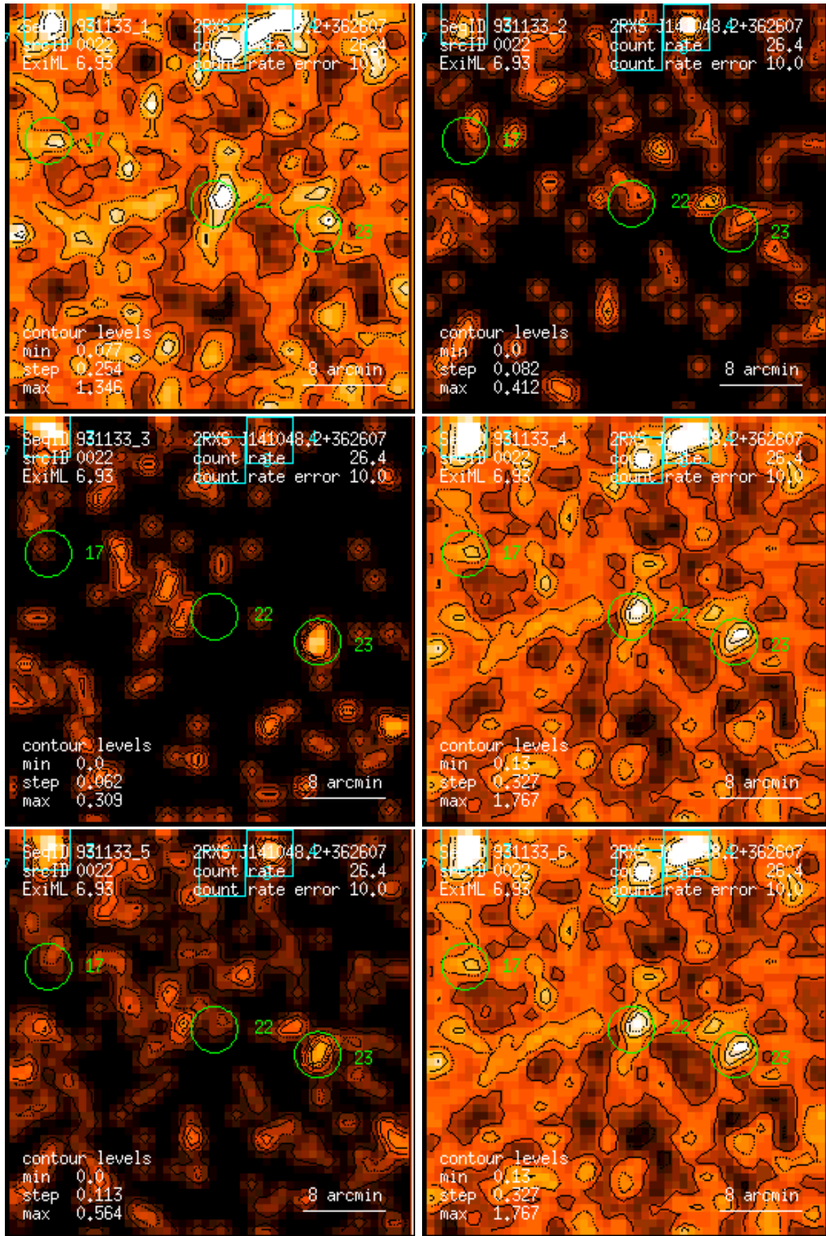
Figure 22: RASS 931133: detection 0022: band rate images, Gaussian filter: (1) PSPC channels 11 – 41, (2) 52 – 90, (3) 91 – 201, (4) 11 – 235, (5) 52 – 201, (6) 11 – 201. Broad band rates in counts/ks. Band rate contour levels in counts/ks/arcmin 2 .
