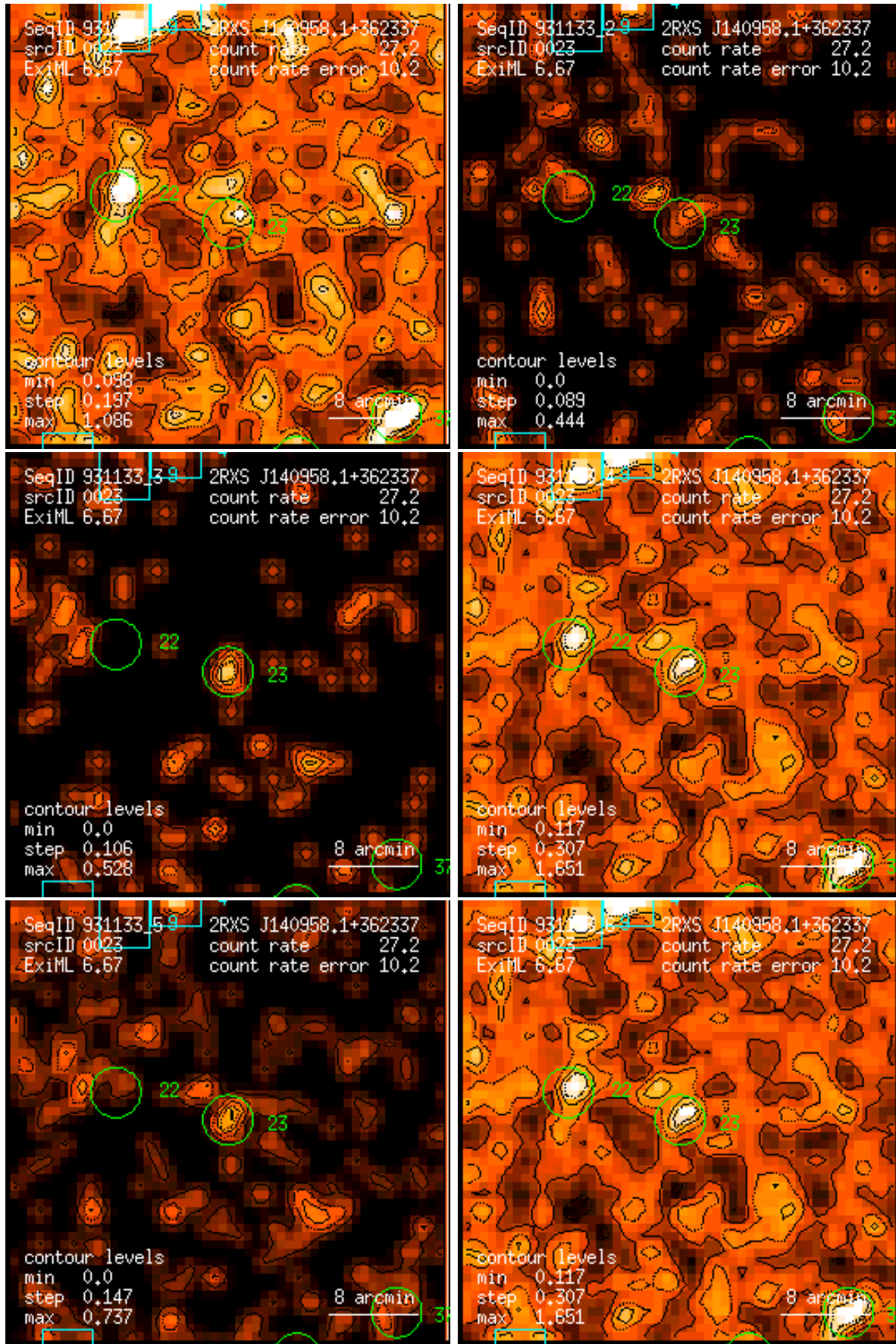
Figure 23: RASS 931133: detection 0023: band rate images, Gaussian filter: (1) PSPC channels 11 – 41, (2) 52 – 90, (3) 91 – 201, (4) 11 – 235, (5) 52 – 201, (6) 11 – 201. Broad band rates in counts/ks. Band rate contour levels in counts/ks/arcmin 2 .
