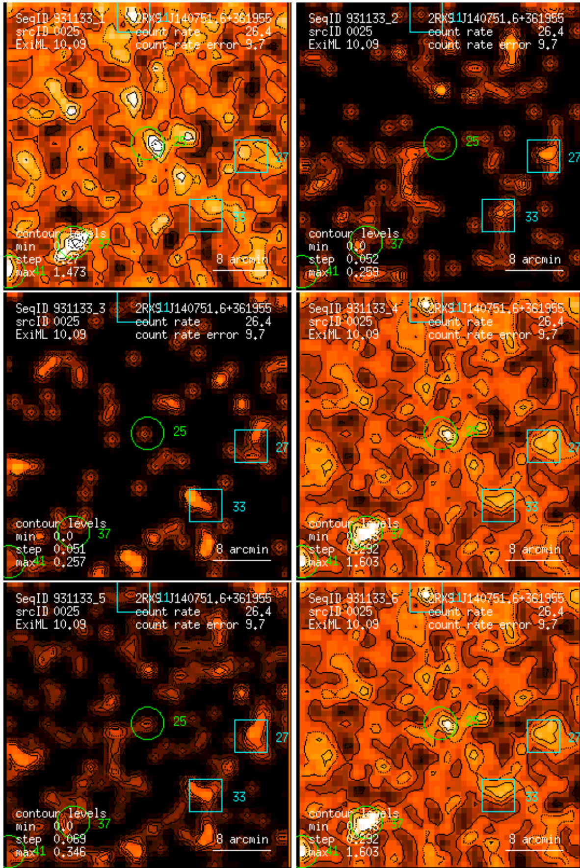
Figure 25: RASS 931133: detection 0025: band rate images, Gaussian filter: (1) PSPC channels 11 – 41, (2) 52 – 90, (3) 91 – 201, (4) 11 – 235, (5) 52 – 201, (6) 11 – 201. Broad band rates in counts/ks. Band rate contour levels in counts/ks/arcmin 2 .
