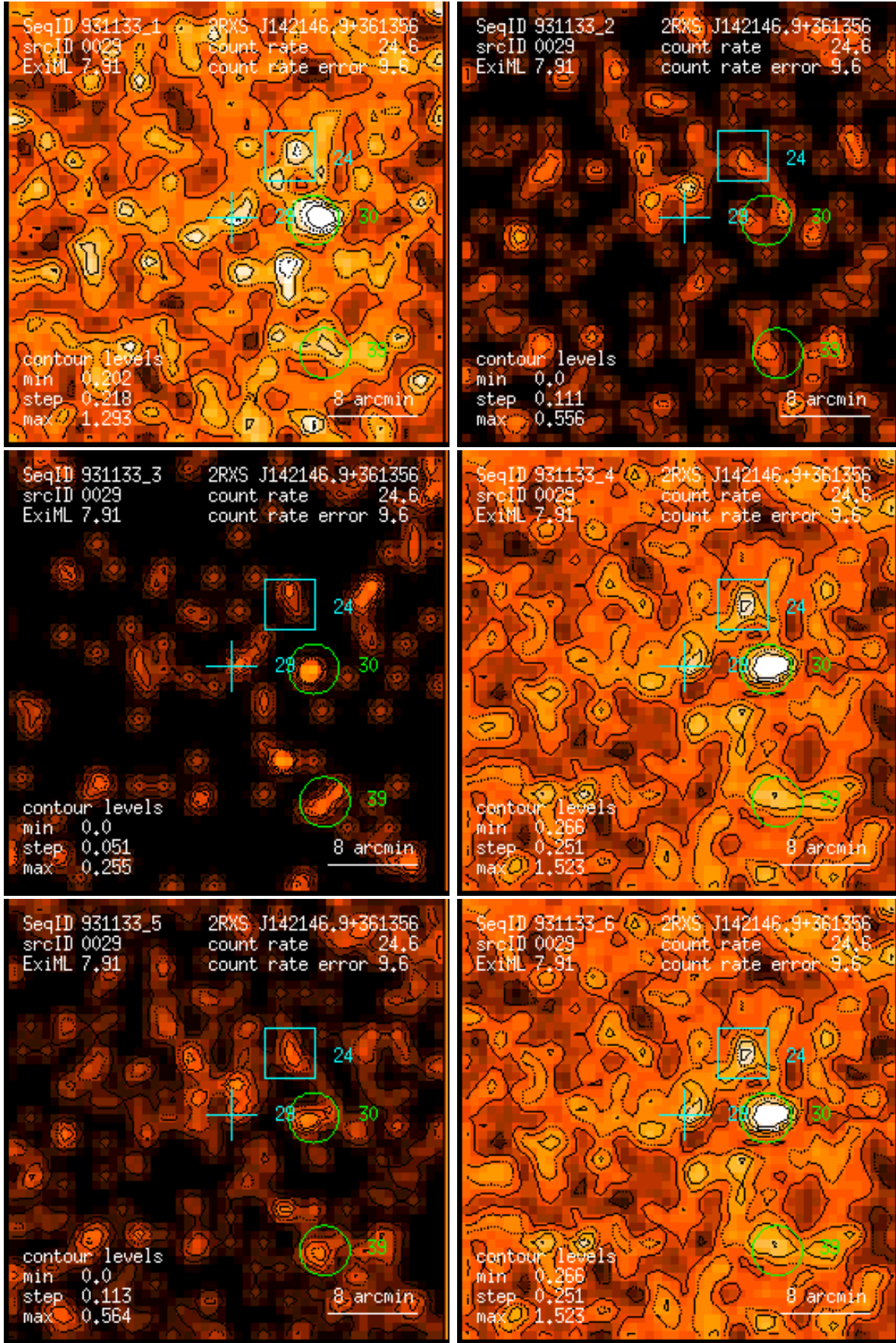
Figure 29: RASS 931133: detection 0029: band rate images, Gaussian filter: (1) PSPC channels 11 – 41, (2) 52 – 90, (3) 91 – 201, (4) 11 – 235, (5) 52 – 201, (6) 11 – 201. Broad band rates in counts/ks. Band rate contour levels in counts/ks/arcmin 2 .
