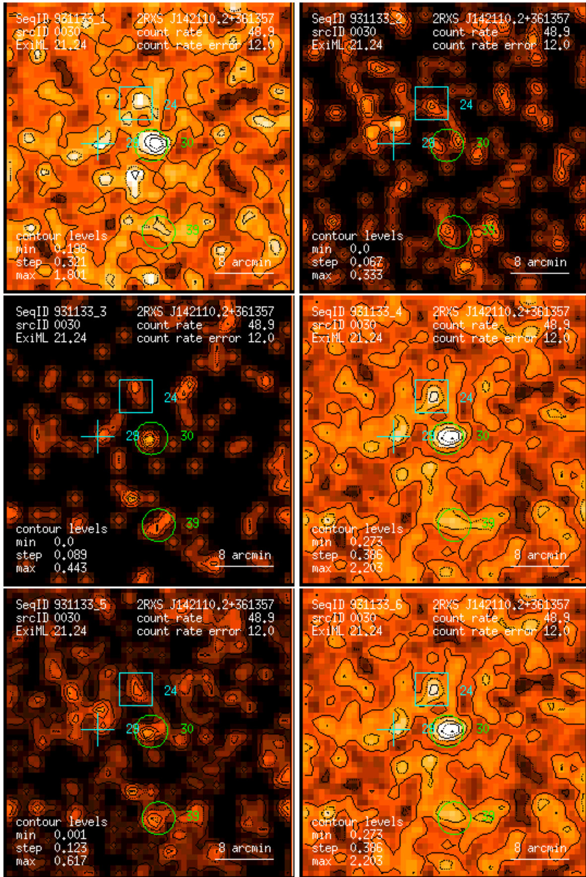
Figure 30: RASS 931133: detection 0030: band rate images, Gaussian filter: (1) PSPC channels 11 – 41, (2) 52 – 90, (3) 91 – 201, (4) 11 – 235, (5) 52 – 201, (6) 11 – 201. Broad band rates in counts/ks. Band rate contour levels in counts/ks/arcmin 2 .
