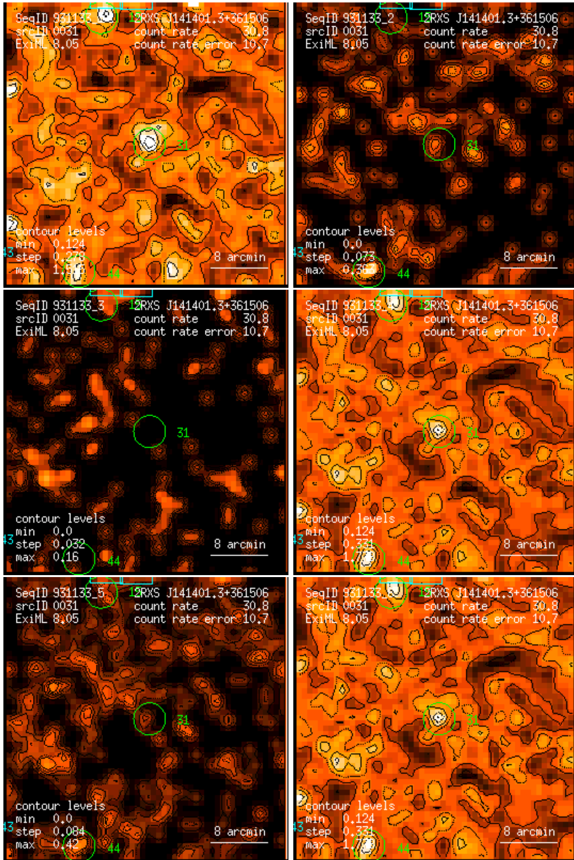
Figure 31: RASS 931133: detection 0031: band rate images, Gaussian filter: (1) PSPC channels 11 – 41, (2) 52 – 90, (3) 91 – 201, (4) 11 – 235, (5) 52 – 201, (6) 11 – 201. Broad band rates in counts/ks. Band rate contour levels in counts/ks/arcmin 2 .
