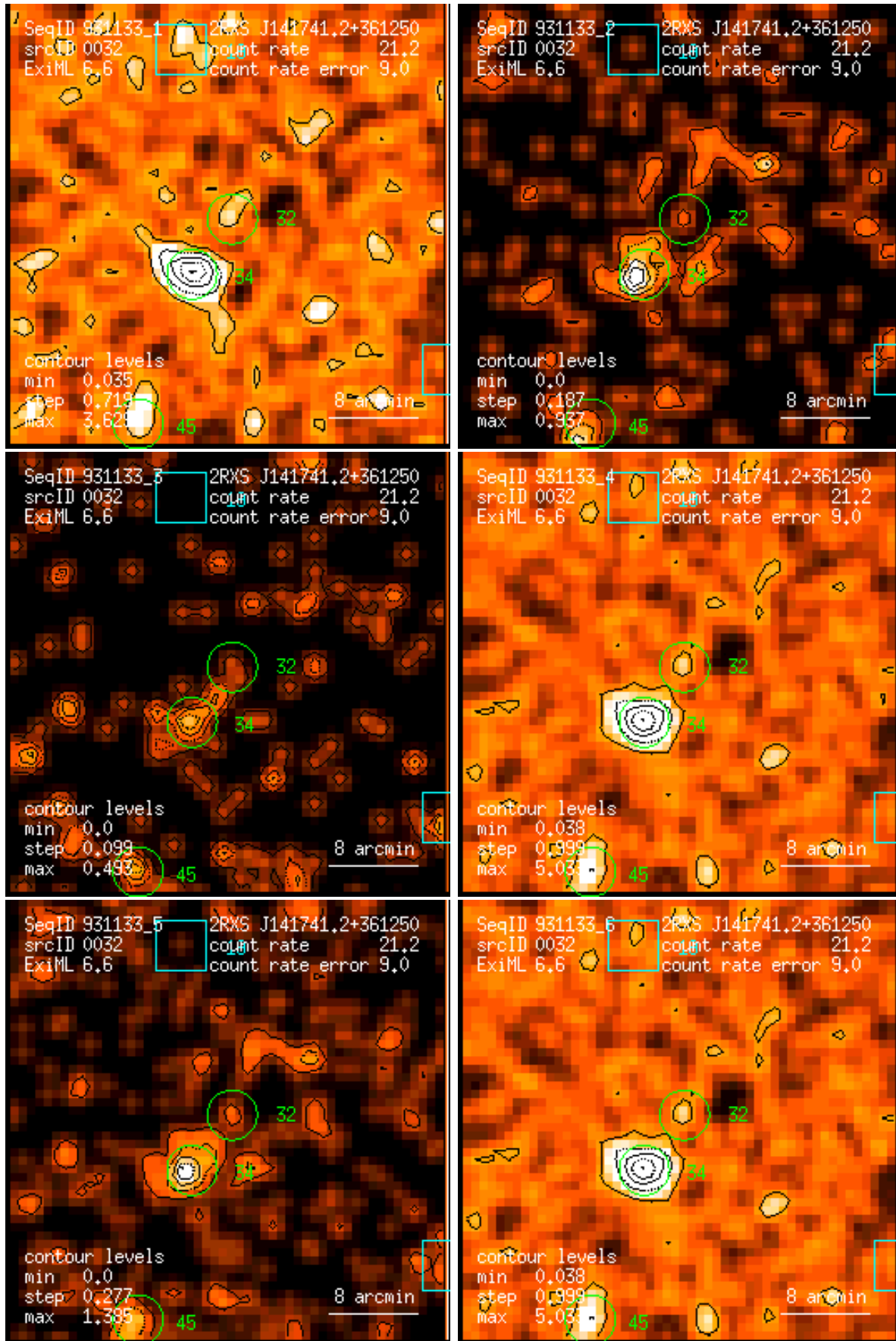
Figure 32: RASS 931133: detection 0032: band rate images, Gaussian filter: (1) PSPC channels 11 – 41, (2) 52 – 90, (3) 91 – 201, (4) 11 – 235, (5) 52 – 201, (6) 11 – 201. Broad band rates in counts/ks. Band rate contour levels in counts/ks/arcmin 2 .
