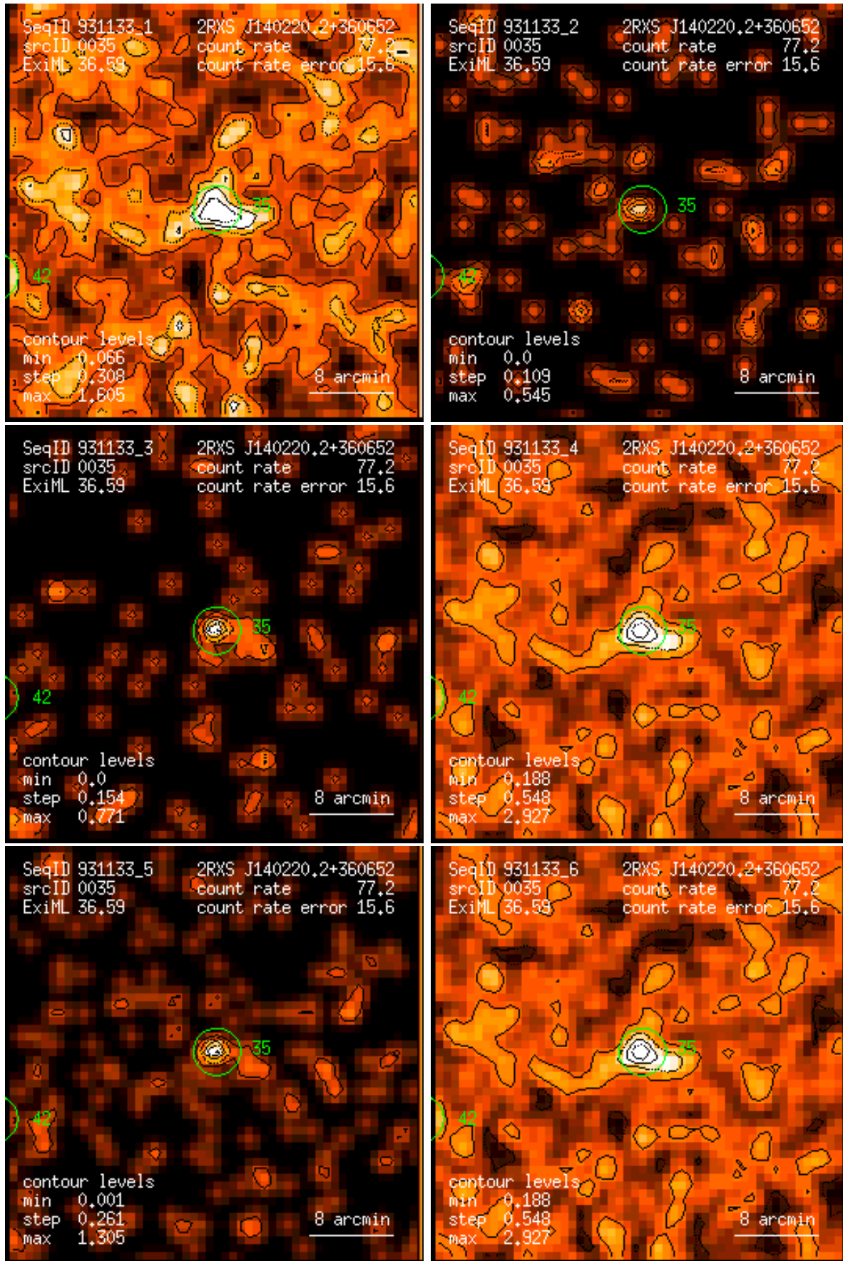
Figure 35: RASS 931133: detection 0035: band rate images, Gaussian filter: (1) PSPC channels 11 – 41, (2) 52 – 90, (3) 91 – 201, (4) 11 – 235, (5) 52 – 201, (6) 11 – 201. Broad band rates in counts/ks. Band rate contour levels in counts/ks/arcmin 2 .
