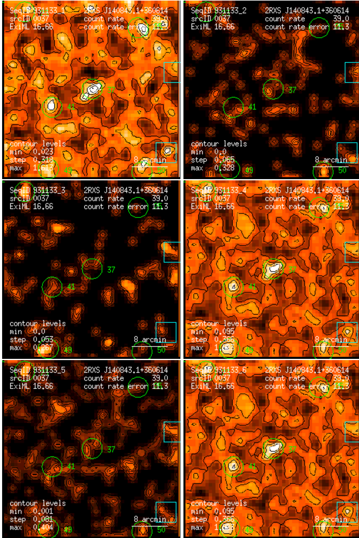
Figure 37: RASS 931133: detection 0037: band rate images, Gaussian filter: (1) PSPC channels 11 – 41, (2) 52 – 90, (3) 91 – 201, (4) 11 – 235, (5) 52 – 201, (6) 11 – 201. Broad band rates in counts/ks. Band rate contour levels in counts/ks/arcmin 2 .
