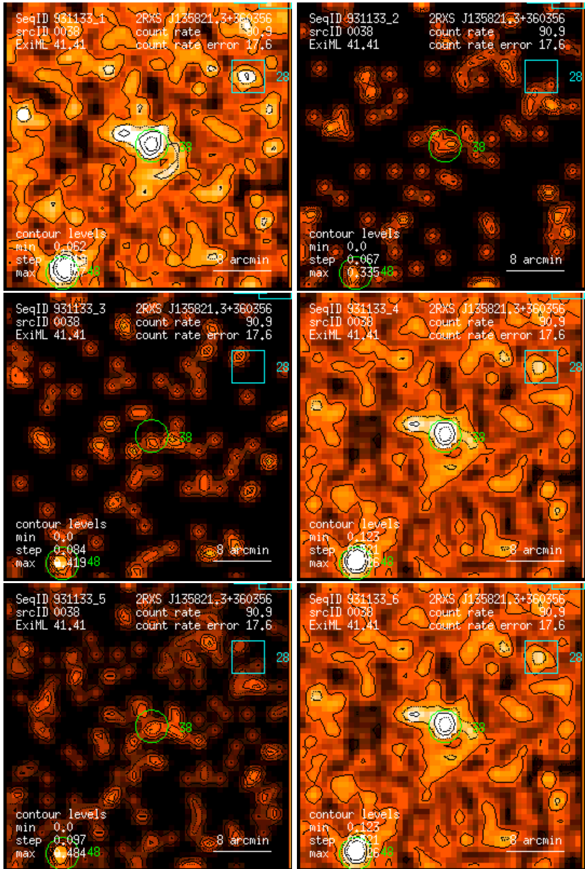
Figure 38: RASS 931133: detection 0038: band rate images, Gaussian filter: (1) PSPC channels 11 – 41, (2) 52 – 90, (3) 91 – 201, (4) 11 – 235, (5) 52 – 201, (6) 11 – 201. Broad band rates in counts/ks. Band rate contour levels in counts/ks/arcmin 2 .
