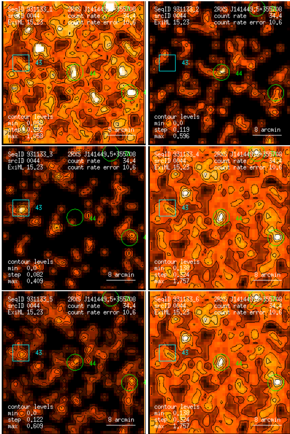
Figure 44: RASS 931133: detection 0044: band rate images, Gaussian filter: (1) PSPC channels 11 – 41, (2) 52 – 90, (3) 91 – 201, (4) 11 – 235, (5) 52 – 201, (6) 11 – 201. Broad band rates in counts/ks. Band rate contour levels in counts/ks/arcmin 2 .
