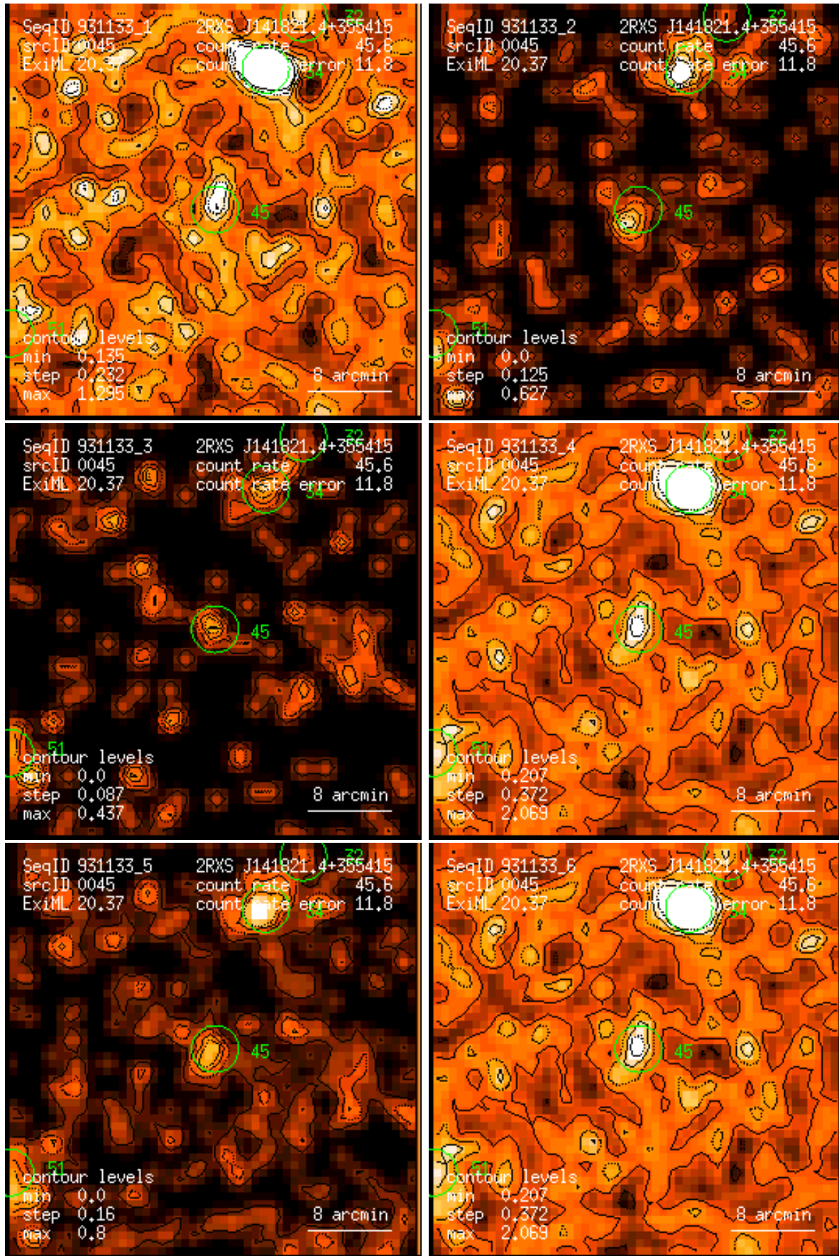
Figure 45: RASS 931133: detection 0045: band rate images, Gaussian filter: (1) PSPC channels 11 – 41, (2) 52 – 90, (3) 91 – 201, (4) 11 – 235, (5) 52 – 201, (6) 11 – 201. Broad band rates in counts/ks. Band rate contour levels in counts/ks/arcmin 2 .
